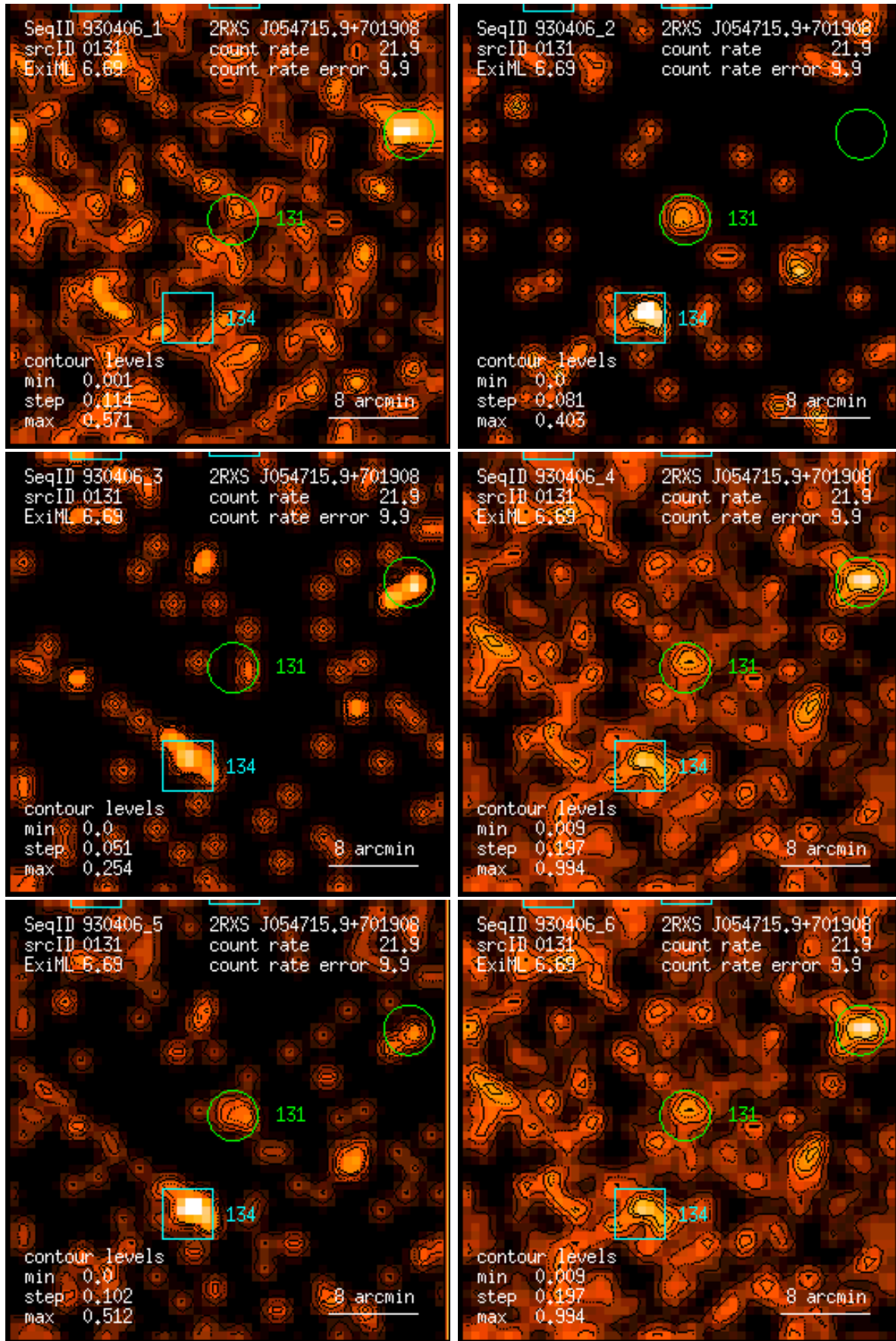
Figure 131: RASS 930406: detection 0131: band rate images, Gaussian filter: (1) PSPC channels 11 – 41, (2) 52 – 90, (3) 91 – 201, (4) 11 – 235, (5) 52 – 201, (6) 11 – 201. Broad band rates in counts/ks. Band rate contour levels in counts/ks/arcmin 2 .
