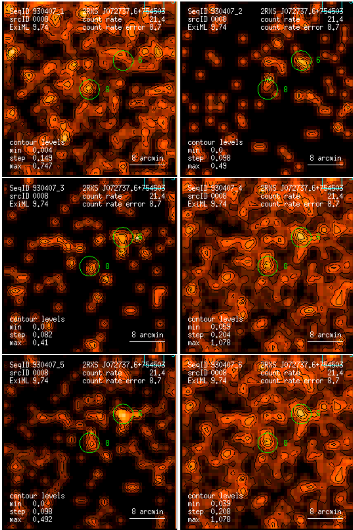
Figure 8: RASS 930407: detection 0008: band rate images, Gaussian filter: (1) PSPC channels 11 – 41, (2) 52 – 90, (3) 91 – 201, (4) 11 – 235, (5) 52 – 201, (6) 11 – 201. Broad band rates in counts/ks. Band rate contour levels in counts/ks/arcmin 2 .
