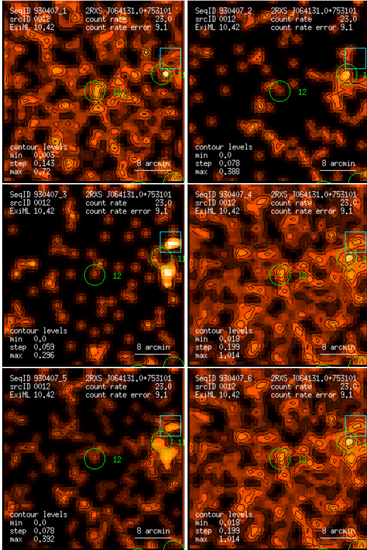
Figure 12: RASS 930407: detection 0012: band rate images, Gaussian filter: (1) PSPC channels 11 – 41, (2) 52 – 90, (3) 91 – 201, (4) 11 – 235, (5) 52 – 201, (6) 11 – 201. Broad band rates in counts/ks. Band rate contour levels in counts/ks/arcmin 2 .
