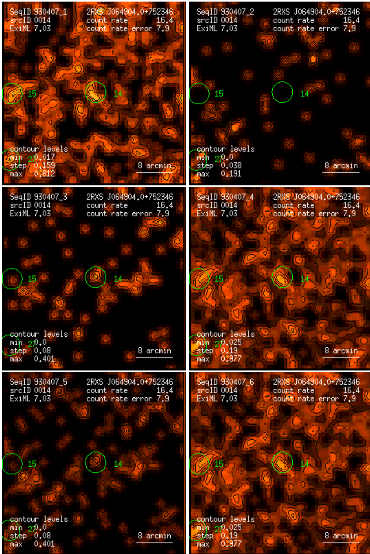
Figure 14: RASS 930407: detection 0014: band rate images, Gaussian filter: (1) PSPC channels 11 – 41, (2) 52 – 90, (3) 91 – 201, (4) 11 – 235, (5) 52 – 201, (6) 11 – 201. Broad band rates in counts/ks. Band rate contour levels in counts/ks/arcmin 2 .
