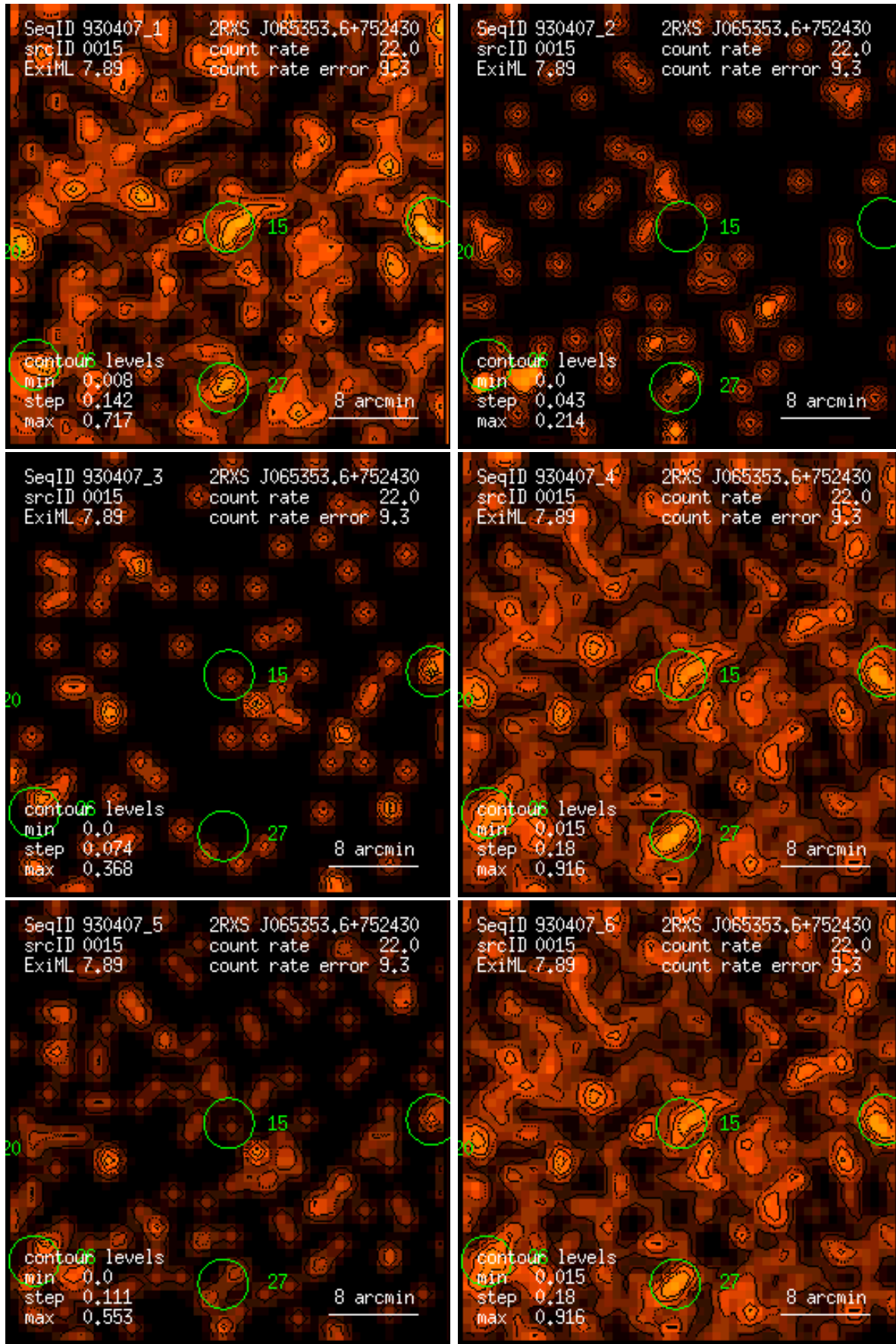
Figure 15: RASS 930407: detection 0015: band rate images, Gaussian filter: (1) PSPC channels 11 – 41, (2) 52 – 90, (3) 91 – 201, (4) 11 – 235, (5) 52 – 201, (6) 11 – 201. Broad band rates in counts/ks. Band rate contour levels in counts/ks/arcmin 2 .
