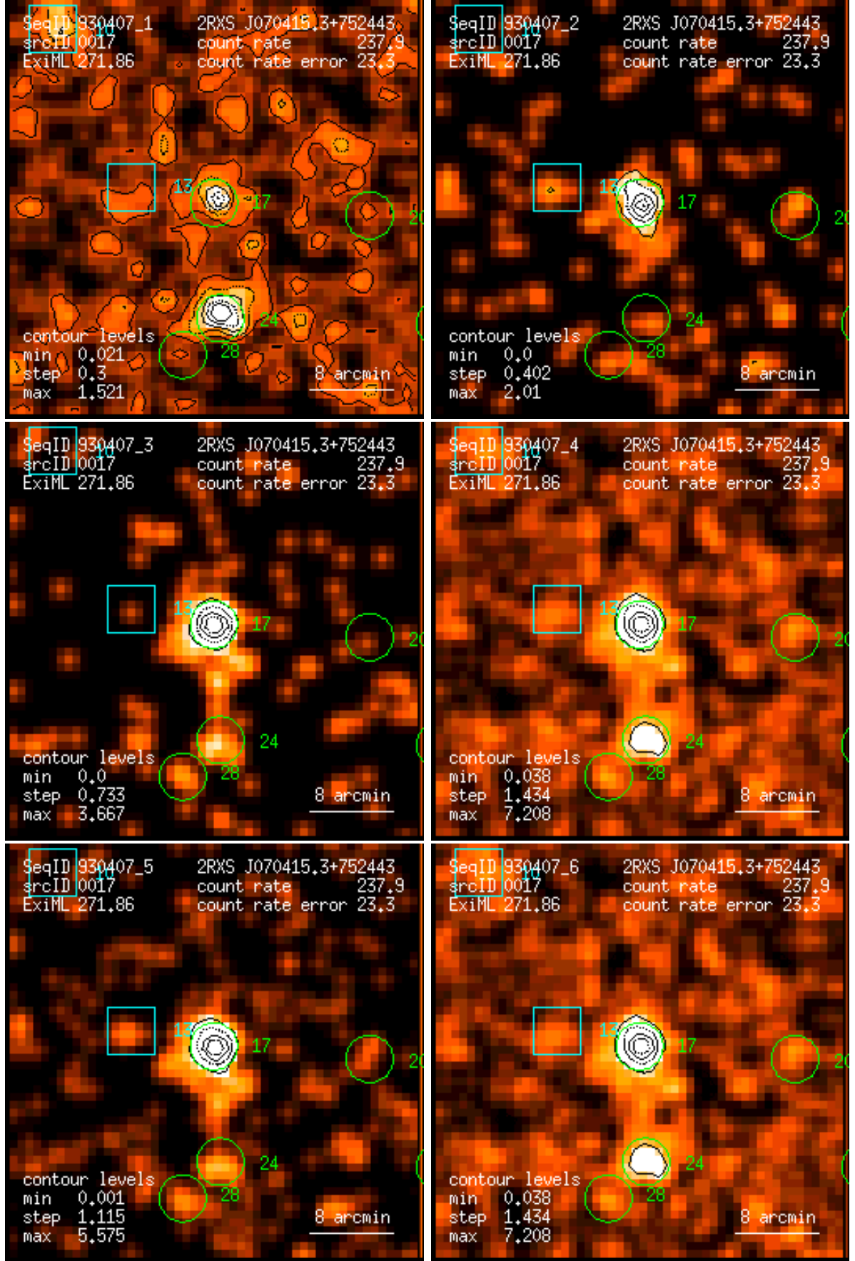
Figure 17: RASS 930407: detection 0017: band rate images, Gaussian filter: (1) PSPC channels 11 – 41, (2) 52 – 90, (3) 91 – 201, (4) 11 – 235, (5) 52 – 201, (6) 11 – 201. Broad band rates in counts/ks. Band rate contour levels in counts/ks/arcmin 2 .
