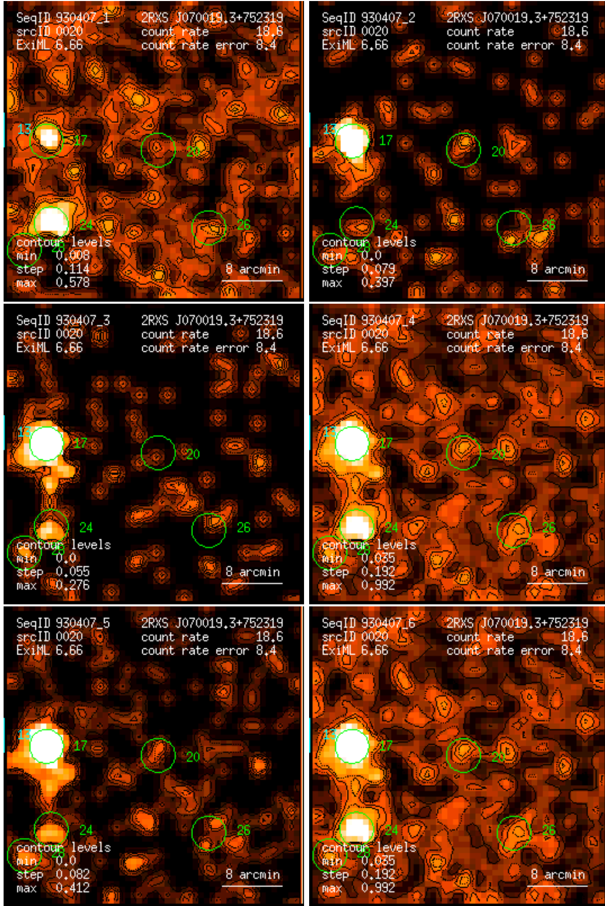
Figure 20: RASS 930407: detection 0020: band rate images, Gaussian filter: (1) PSPC channels 11 – 41, (2) 52 – 90, (3) 91 – 201, (4) 11 – 235, (5) 52 – 201, (6) 11 – 201. Broad band rates in counts/ks. Band rate contour levels in counts/ks/arcmin 2 .
