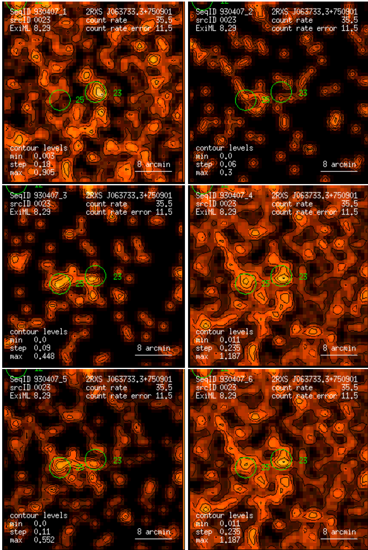
Figure 23: RASS 930407: detection 0023: band rate images, Gaussian filter: (1) PSPC channels 11 – 41, (2) 52 – 90, (3) 91 – 201, (4) 11 – 235, (5) 52 – 201, (6) 11 – 201. Broad band rates in counts/ks. Band rate contour levels in counts/ks/arcmin 2 .
