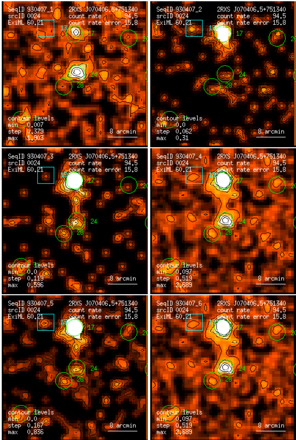
Figure 24: RASS 930407: detection 0024: band rate images, Gaussian filter: (1) PSPC channels 11 – 41, (2) 52 – 90, (3) 91 – 201, (4) 11 – 235, (5) 52 – 201, (6) 11 – 201. Broad band rates in counts/ks. Band rate contour levels in counts/ks/arcmin 2 .
