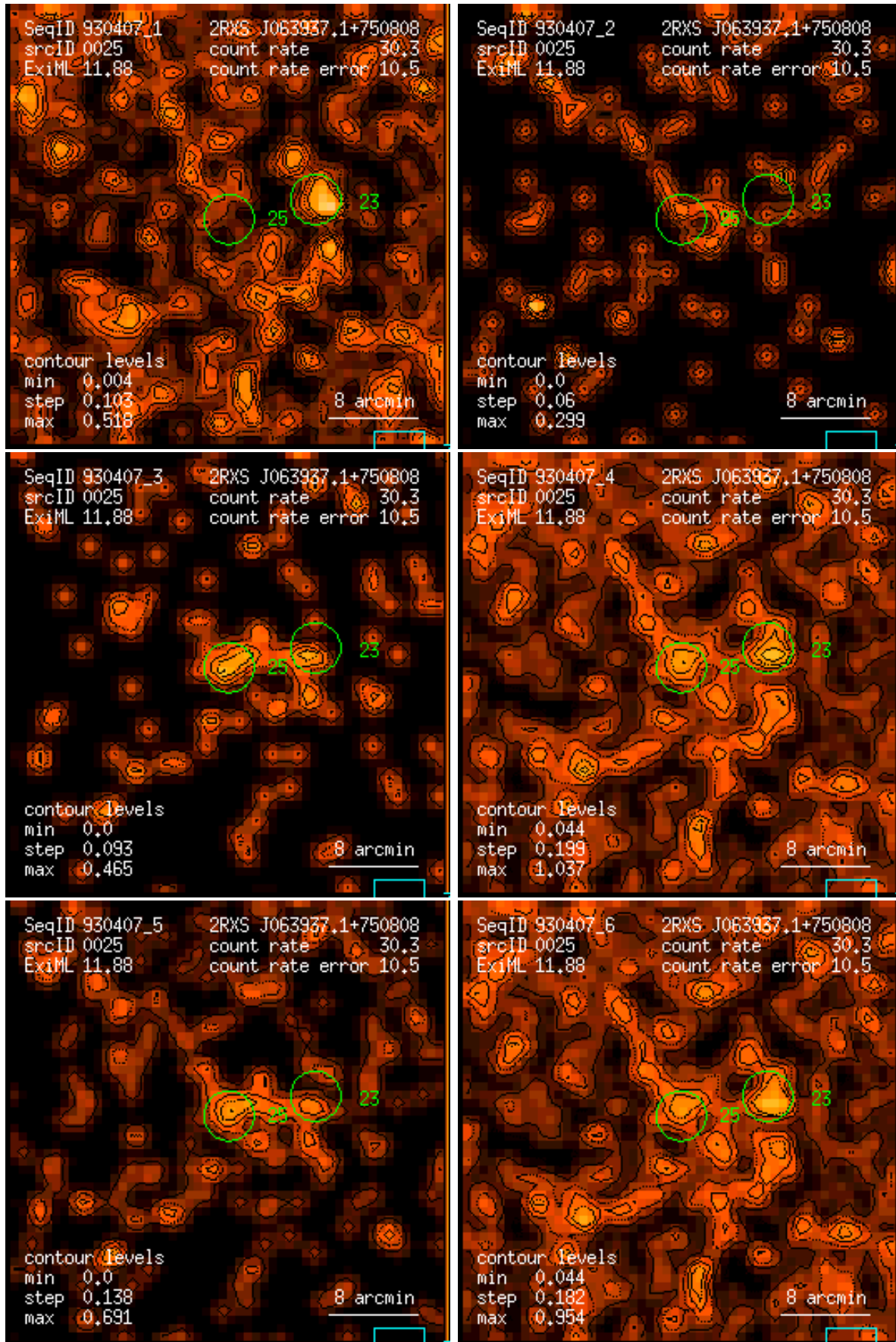
Figure 25: RASS 930407: detection 0025: band rate images, Gaussian filter: (1) PSPC channels 11 – 41, (2) 52 – 90, (3) 91 – 201, (4) 11 – 235, (5) 52 – 201, (6) 11 – 201. Broad band rates in counts/ks. Band rate contour levels in counts/ks/arcmin 2 .
