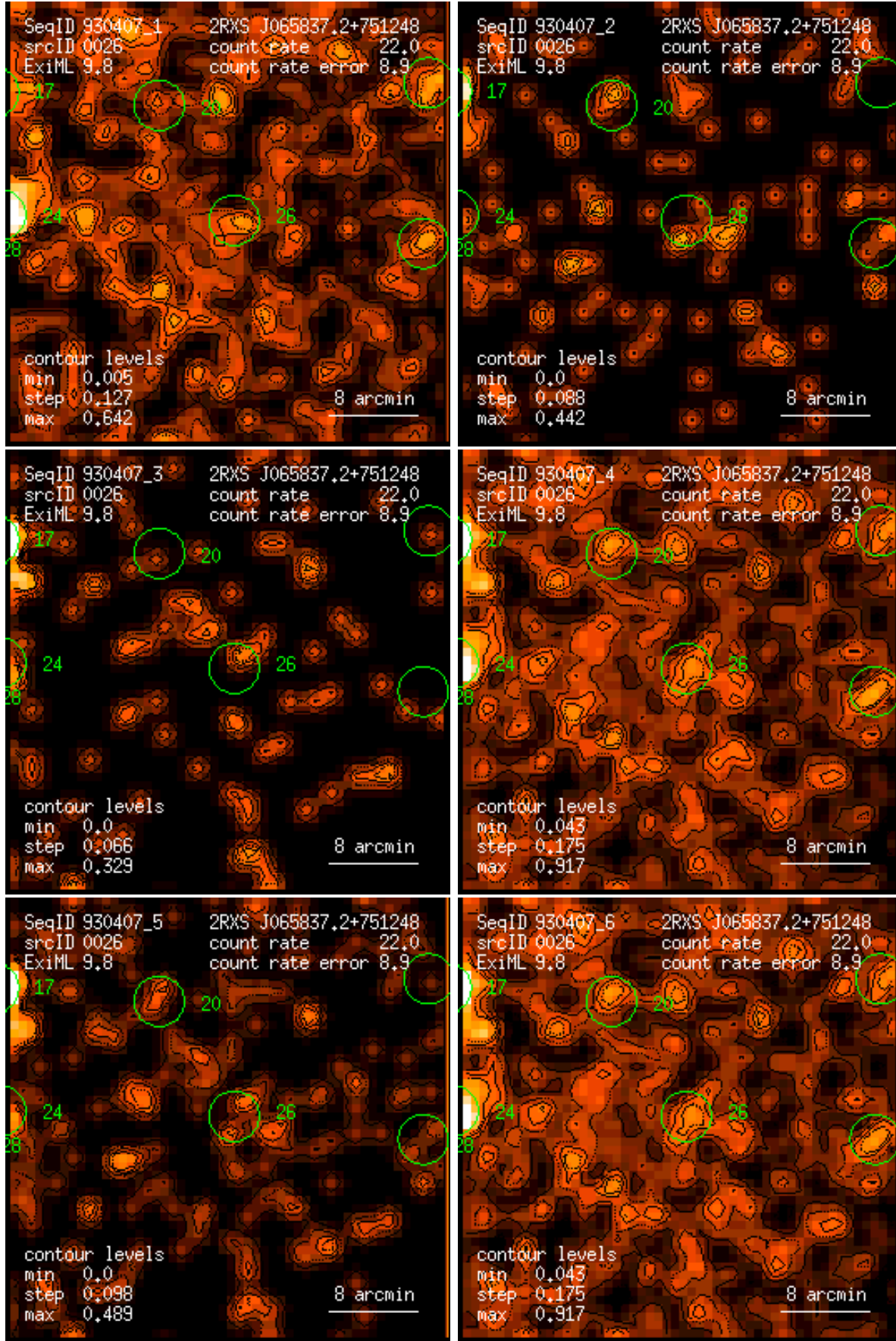
Figure 26: RASS 930407: detection 0026: band rate images, Gaussian filter: (1) PSPC channels 11 – 41, (2) 52 – 90, (3) 91 – 201, (4) 11 – 235, (5) 52 – 201, (6) 11 – 201. Broad band rates in counts/ks. Band rate contour levels in counts/ks/arcmin 2 .
