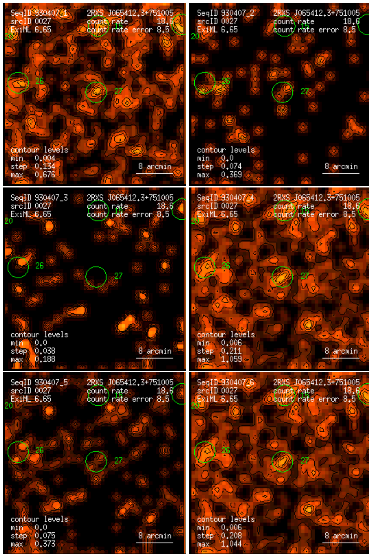
Figure 27: RASS 930407: detection 0027: band rate images, Gaussian filter: (1) PSPC channels 11 – 41, (2) 52 – 90, (3) 91 – 201, (4) 11 – 235, (5) 52 – 201, (6) 11 – 201. Broad band rates in counts/ks. Band rate contour levels in counts/ks/arcmin 2 .
