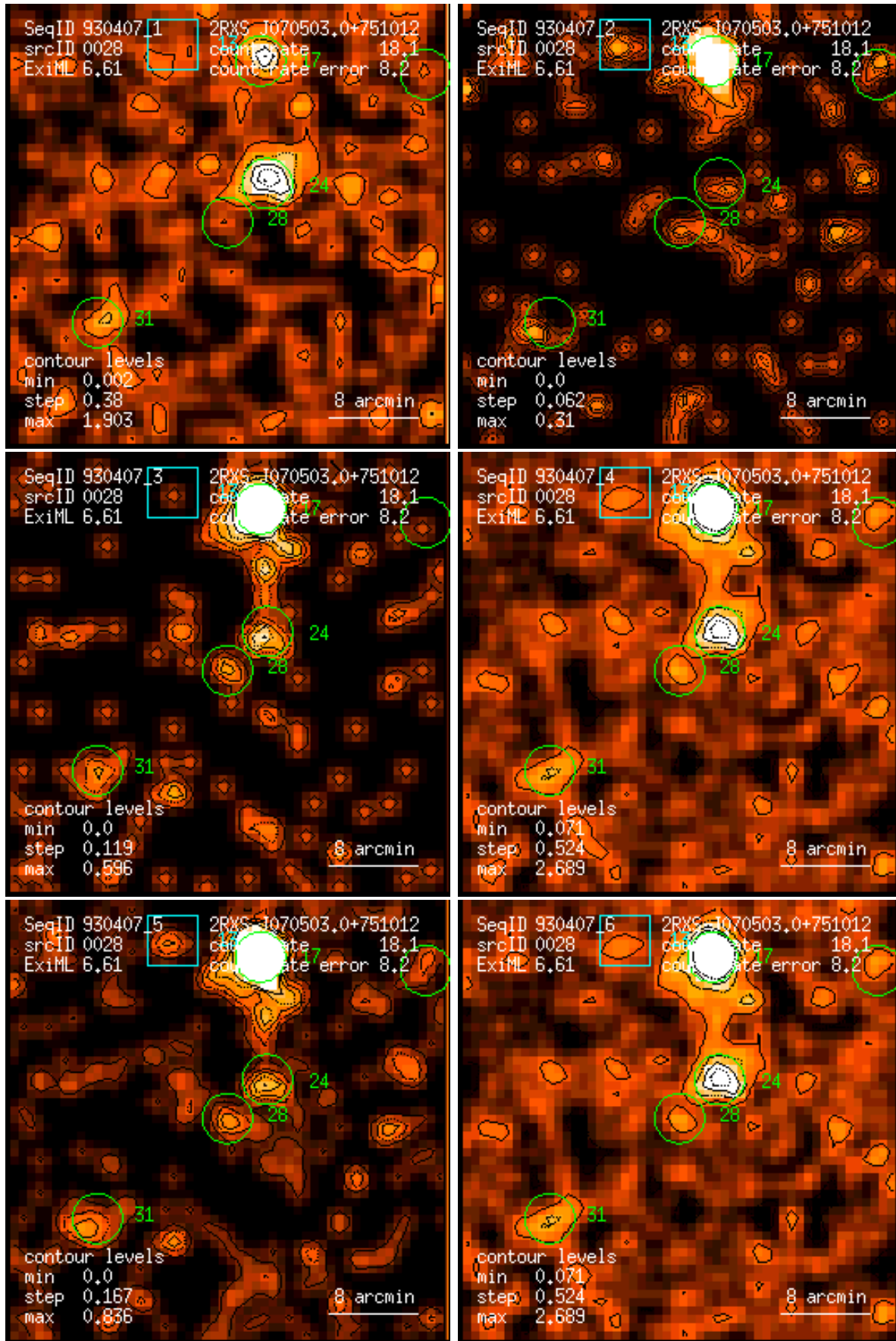
Figure 28: RASS 930407: detection 0028: band rate images, Gaussian filter: (1) PSPC channels 11 – 41, (2) 52 – 90, (3) 91 – 201, (4) 11 – 235, (5) 52 – 201, (6) 11 – 201. Broad band rates in counts/ks. Band rate contour levels in counts/ks/arcmin 2 .
