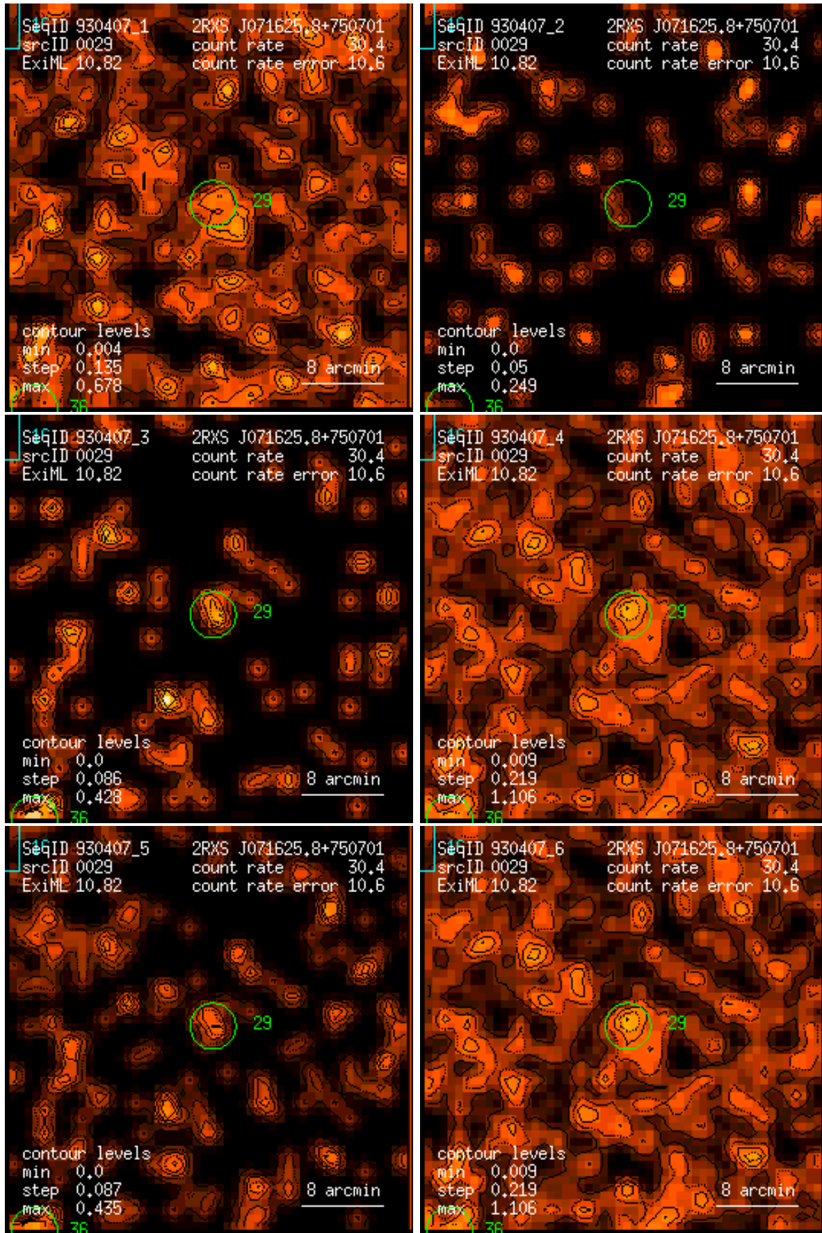
Figure 29: RASS 930407: detection 0029: band rate images, Gaussian filter: (1) PSPC channels 11 – 41, (2) 52 – 90, (3) 91 – 201, (4) 11 – 235, (5) 52 – 201, (6) 11 – 201. Broad band rates in counts/ks. Band rate contour levels in counts/ks/arcmin 2 .
