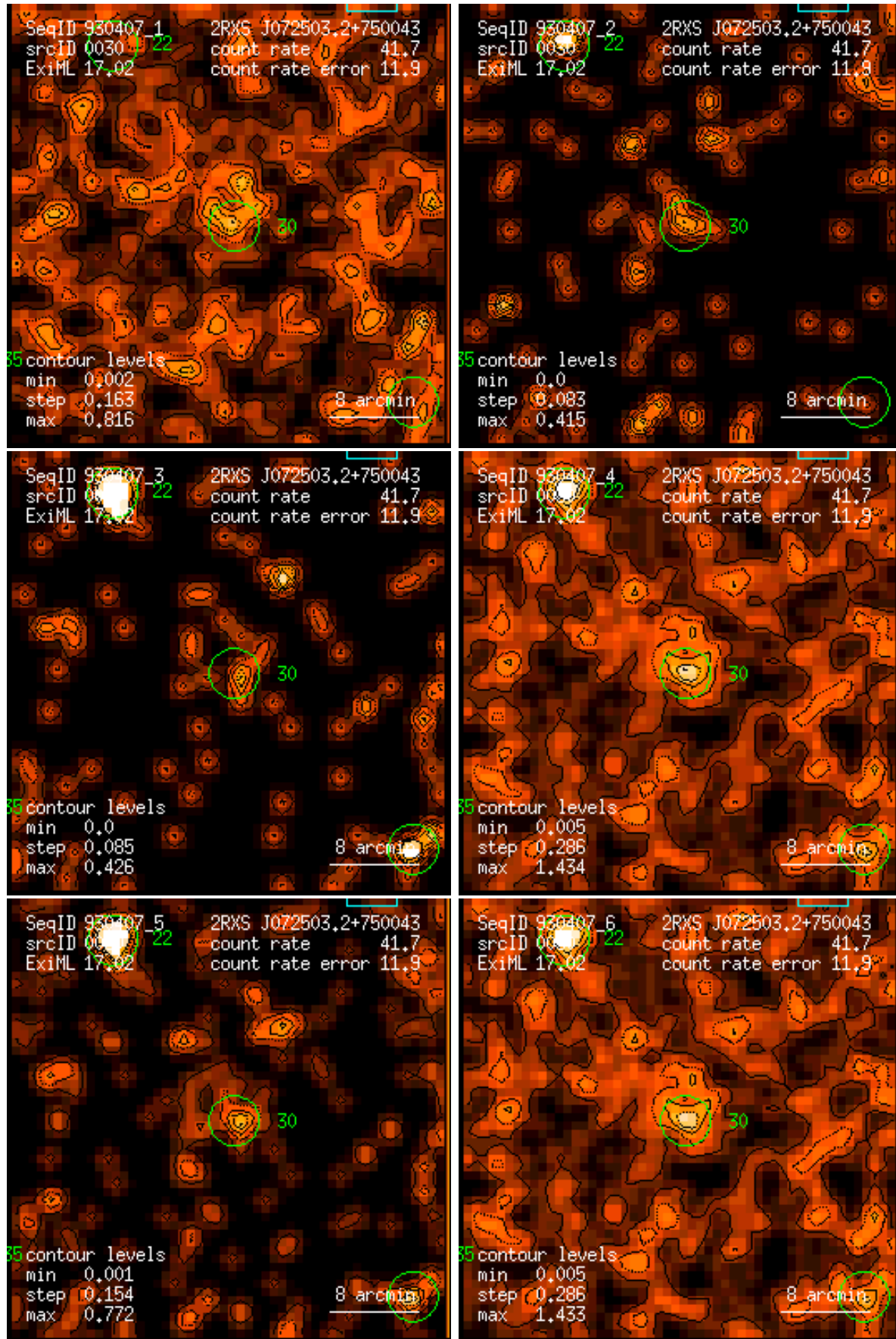
Figure 30: RASS 930407: detection 0030: band rate images, Gaussian filter: (1) PSPC channels 11 – 41, (2) 52 – 90, (3) 91 – 201, (4) 11 – 235, (5) 52 – 201, (6) 11 – 201. Broad band rates in counts/ks. Band rate contour levels in counts/ks/arcmin 2 .
