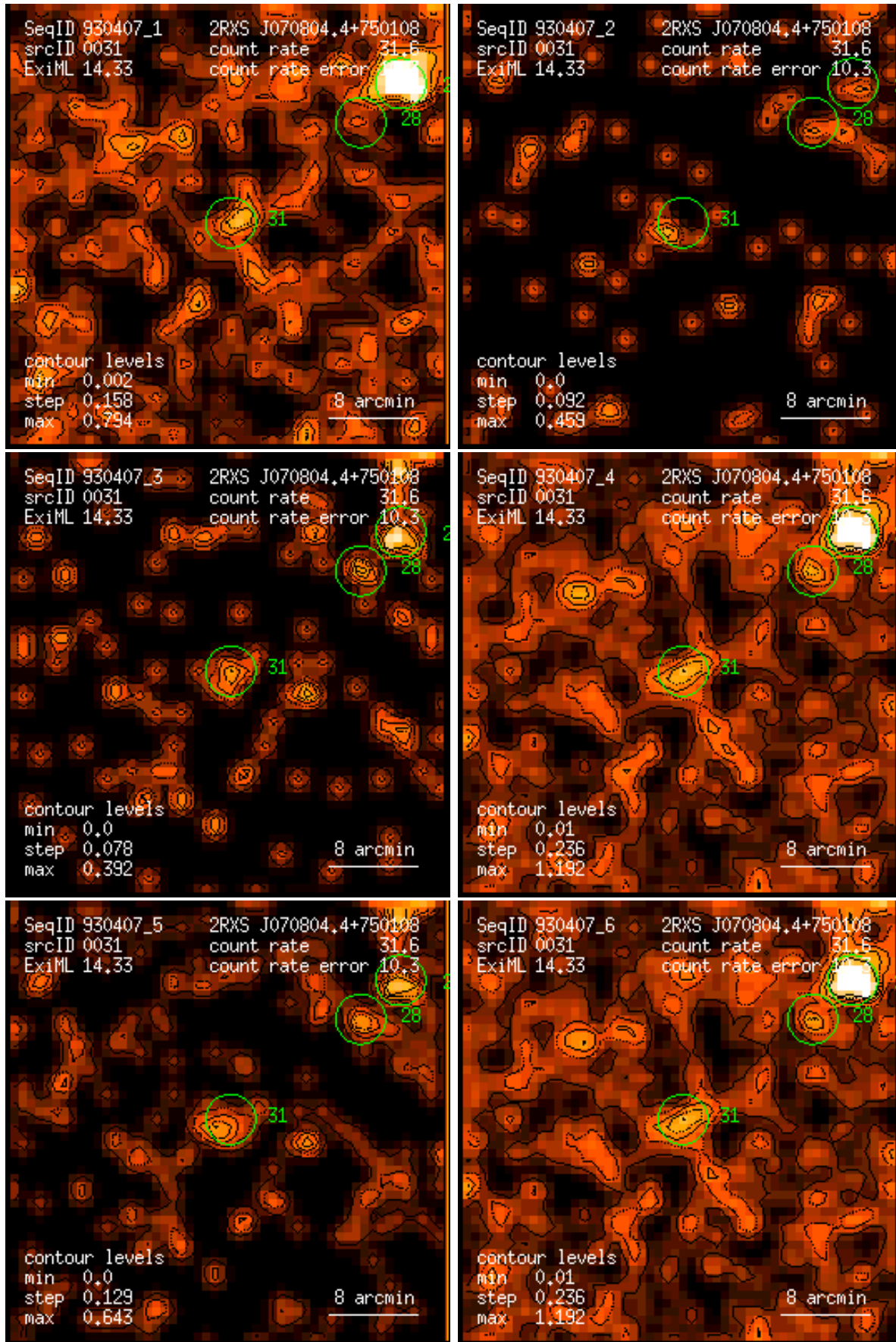
Figure 31: RASS 930407: detection 0031: band rate images, Gaussian filter: (1) PSPC channels 11 – 41, (2) 52 – 90, (3) 91 – 201, (4) 11 – 235, (5) 52 – 201, (6) 11 – 201. Broad band rates in counts/ks. Band rate contour levels in counts/ks/arcmin 2 .
