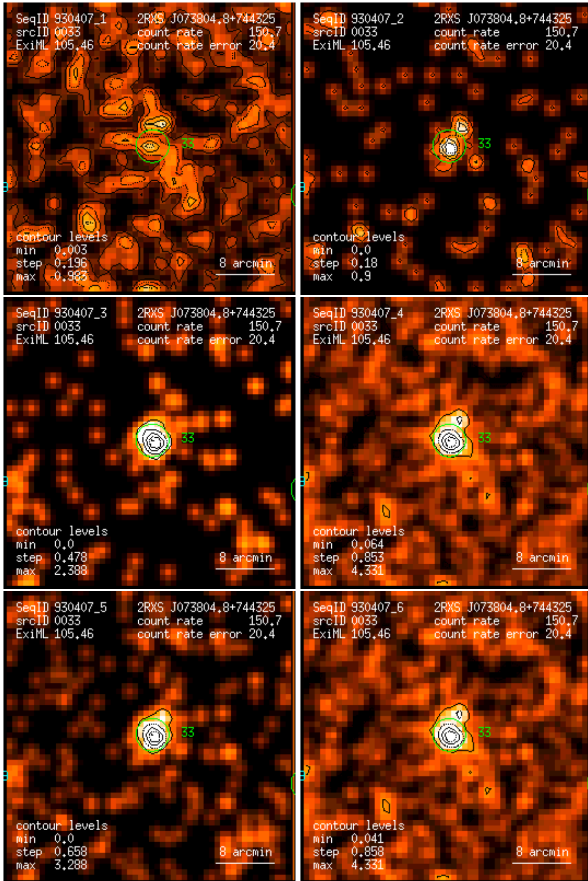
Figure 33: RASS 930407: detection 0033: band rate images, Gaussian filter: (1) PSPC channels 11 – 41, (2) 52 – 90, (3) 91 – 201, (4) 11 – 235, (5) 52 – 201, (6) 11 – 201. Broad band rates in counts/ks. Band rate contour levels in counts/ks/arcmin 2 .
