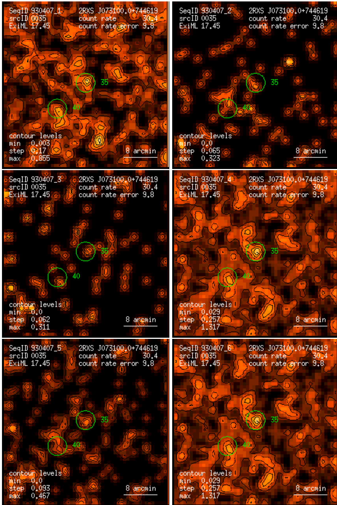
Figure 35: RASS 930407: detection 0035: band rate images, Gaussian filter: (1) PSPC channels 11 – 41, (2) 52 – 90, (3) 91 – 201, (4) 11 – 235, (5) 52 – 201, (6) 11 – 201. Broad band rates in counts/ks. Band rate contour levels in counts/ks/arcmin 2 .
