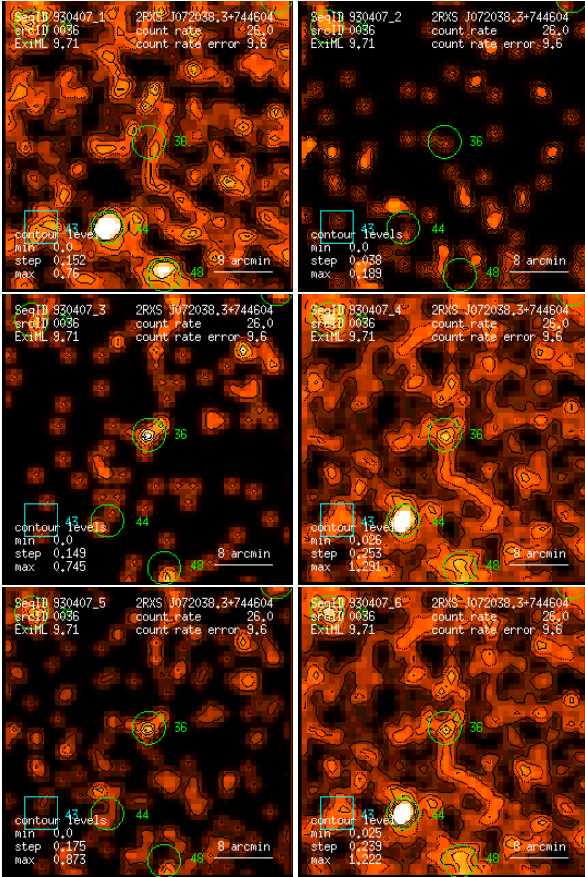
Figure 36: RASS 930407: detection 0036: band rate images, Gaussian filter: (1) PSPC channels 11 – 41, (2) 52 – 90, (3) 91 – 201, (4) 11 – 235, (5) 52 – 201, (6) 11 – 201. Broad band rates in counts/ks. Band rate contour levels in counts/ks/arcmin 2 .
