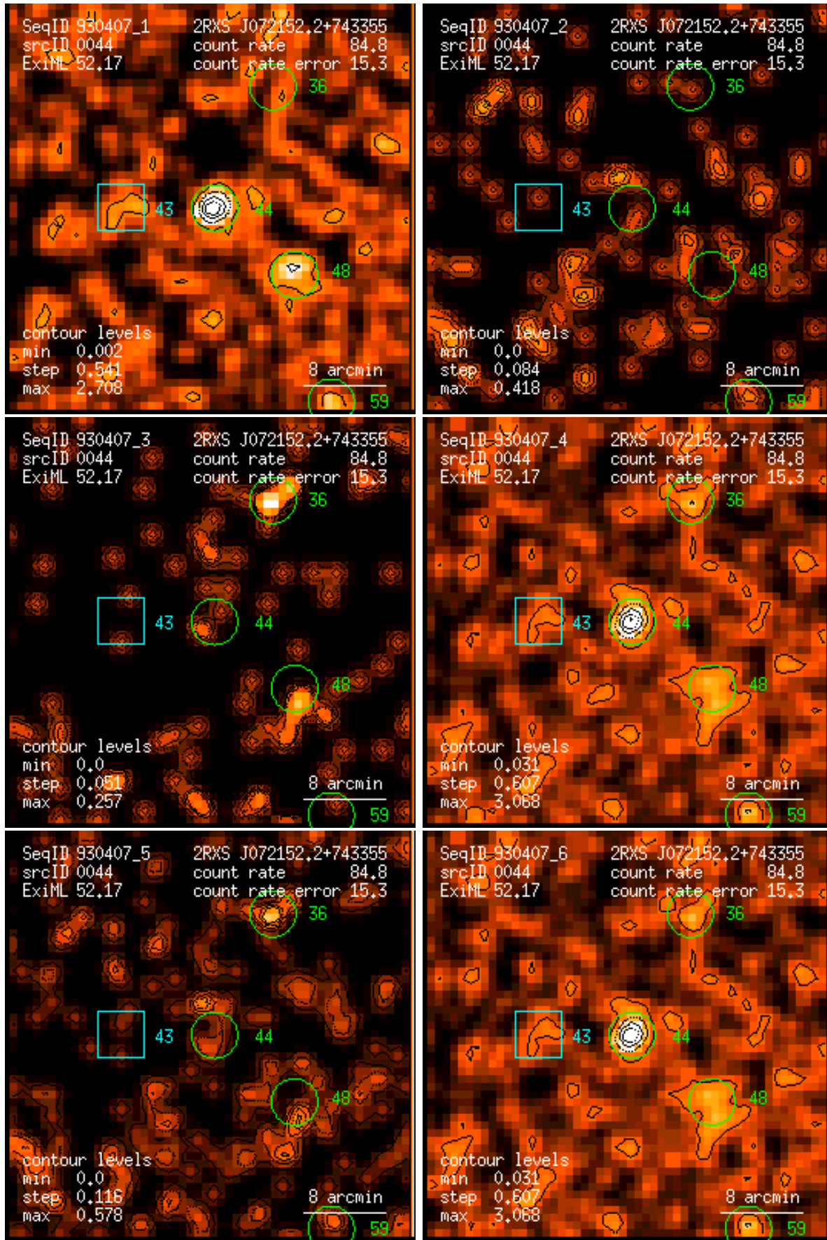
Figure 44: RASS 930407: detection 0044: band rate images, Gaussian filter: (1) PSPC channels 11 – 41, (2) 52 – 90, (3) 91 – 201, (4) 11 – 235, (5) 52 – 201, (6) 11 – 201. Broad band rates in counts/ks. Band rate contour levels in counts/ks/arcmin 2 .
