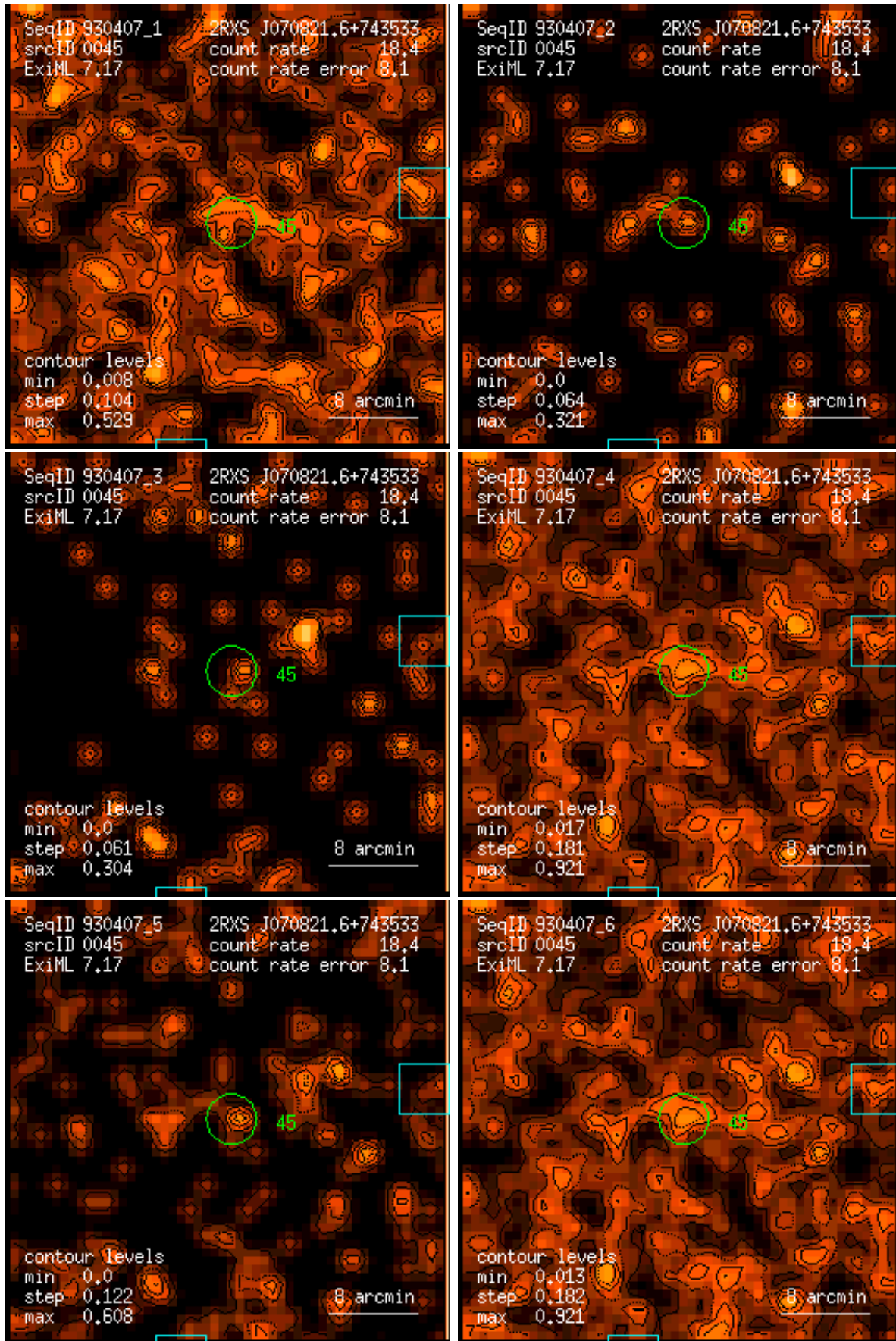
Figure 45: RASS 930407: detection 0045: band rate images, Gaussian filter: (1) PSPC channels 11 – 41, (2) 52 – 90, (3) 91 – 201, (4) 11 – 235, (5) 52 – 201, (6) 11 – 201. Broad band rates in counts/ks. Band rate contour levels in counts/ks/arcmin 2 .
