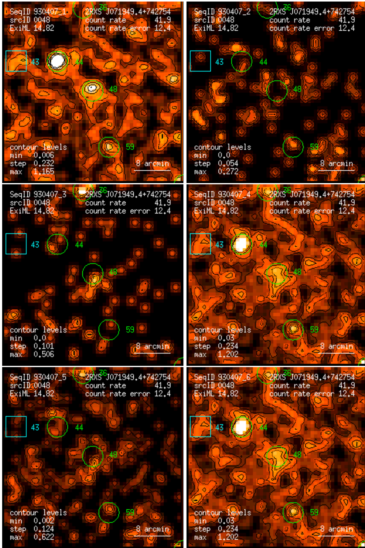
Figure 48: RASS 930407: detection 0048: band rate images, Gaussian filter: (1) PSPC channels 11 – 41, (2) 52 – 90, (3) 91 – 201, (4) 11 – 235, (5) 52 – 201, (6) 11 – 201. Broad band rates in counts/ks. Band rate contour levels in counts/ks/arcmin 2 .
