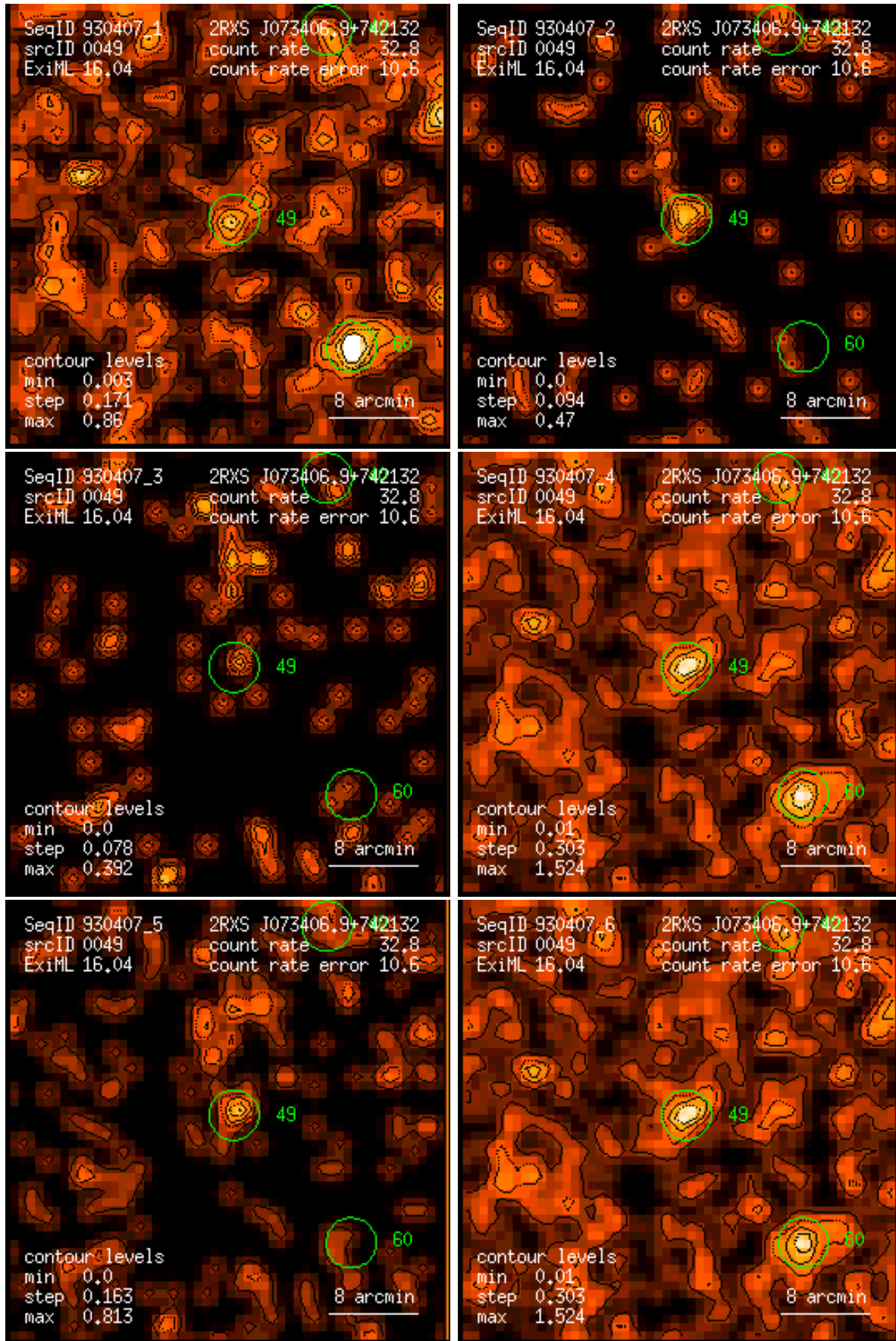
Figure 49: RASS 930407: detection 0049: band rate images, Gaussian filter: (1) PSPC channels 11 – 41, (2) 52 – 90, (3) 91 – 201, (4) 11 – 235, (5) 52 – 201, (6) 11 – 201. Broad band rates in counts/ks. Band rate contour levels in counts/ks/arcmin 2 .
