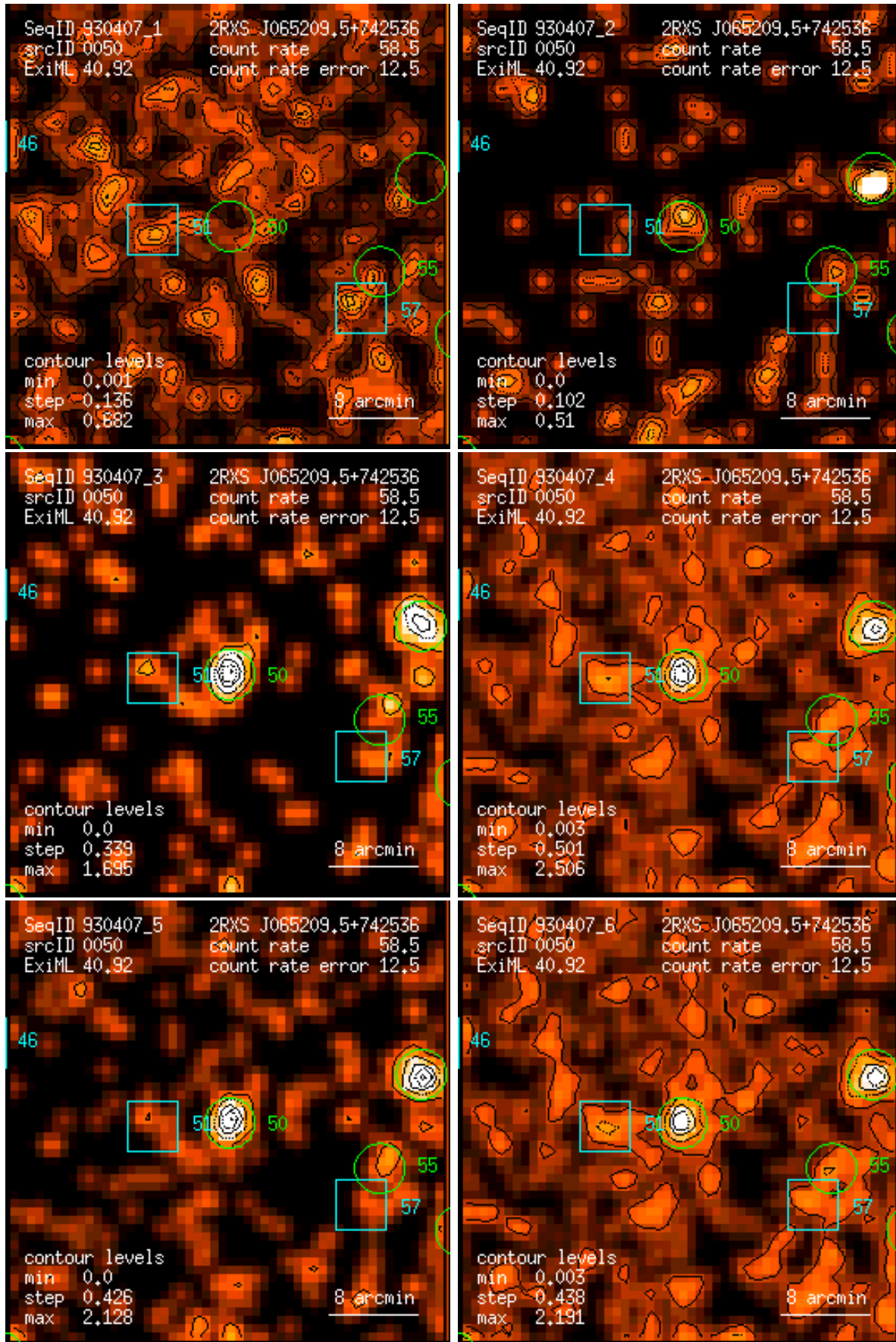
Figure 50: RASS 930407: detection 0050: band rate images, Gaussian filter: (1) PSPC channels 11 – 41, (2) 52 – 90, (3) 91 – 201, (4) 11 – 235, (5) 52 – 201, (6) 11 – 201. Broad band rates in counts/ks. Band rate contour levels in counts/ks/arcmin 2 .
