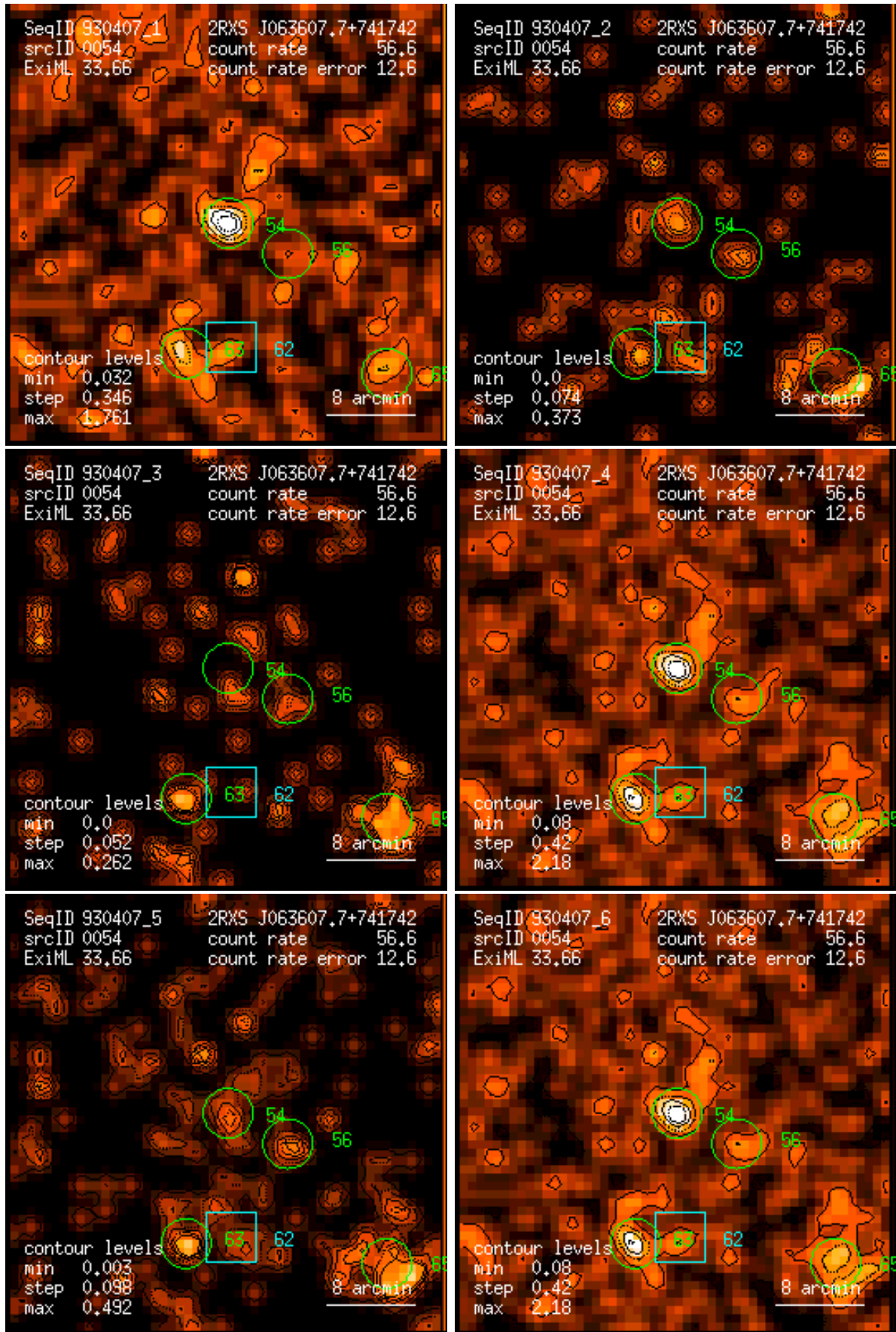
Figure 54: RASS 930407: detection 0054: band rate images, Gaussian filter: (1) PSPC channels 11 – 41, (2) 52 – 90, (3) 91 – 201, (4) 11 – 235, (5) 52 – 201, (6) 11 – 201. Broad band rates in counts/ks. Band rate contour levels in counts/ks/arcmin 2 .
