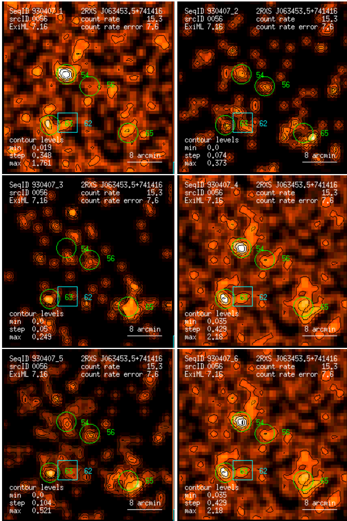
Figure 56: RASS 930407: detection 0056: band rate images, Gaussian filter: (1) PSPC channels 11 – 41, (2) 52 – 90, (3) 91 – 201, (4) 11 – 235, (5) 52 – 201, (6) 11 – 201. Broad band rates in counts/ks. Band rate contour levels in counts/ks/arcmin 2 .
