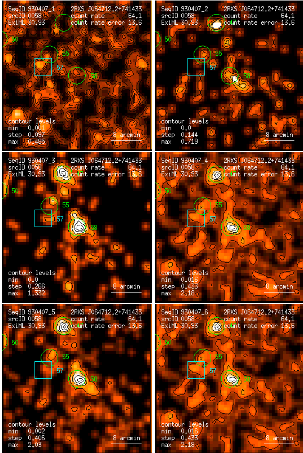
Figure 58: RASS 930407: detection 0058: band rate images, Gaussian filter: (1) PSPC channels 11 – 41, (2) 52 – 90, (3) 91 – 201, (4) 11 – 235, (5) 52 – 201, (6) 11 – 201. Broad band rates in counts/ks. Band rate contour levels in counts/ks/arcmin 2 .
