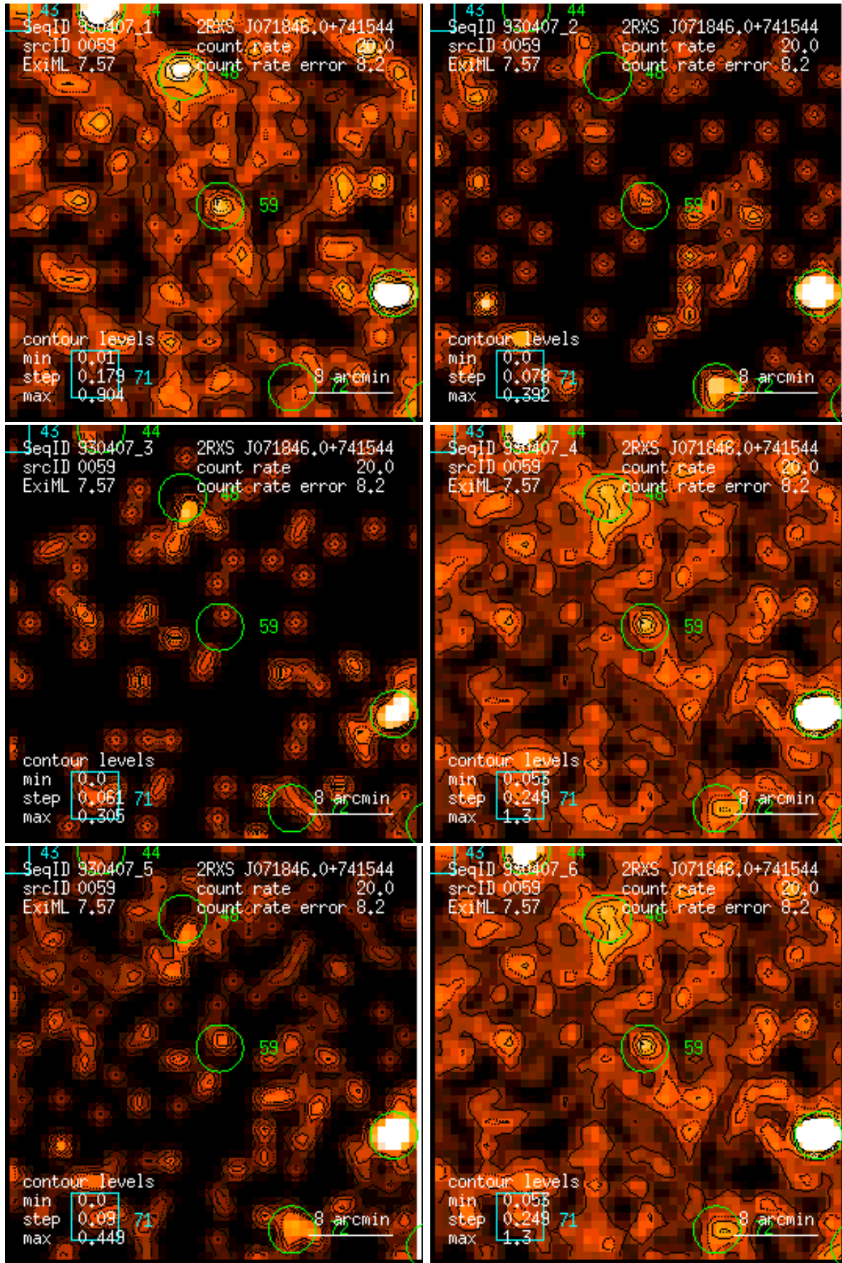
Figure 59: RASS 930407: detection 0059: band rate images, Gaussian filter: (1) PSPC channels 11 – 41, (2) 52 – 90, (3) 91 – 201, (4) 11 – 235, (5) 52 – 201, (6) 11 – 201. Broad band rates in counts/ks. Band rate contour levels in counts/ks/arcmin 2 .
