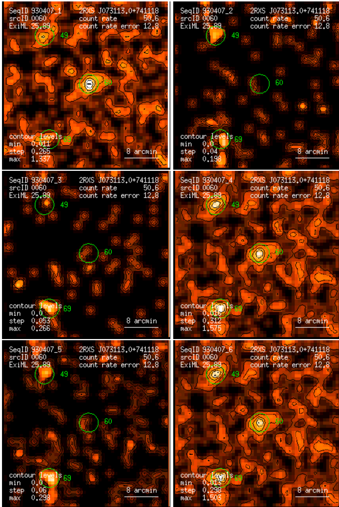
Figure 60: RASS 930407: detection 0060: band rate images, Gaussian filter: (1) PSPC channels 11 – 41, (2) 52 – 90, (3) 91 – 201, (4) 11 – 235, (5) 52 – 201, (6) 11 – 201. Broad band rates in counts/ks. Band rate contour levels in counts/ks/arcmin 2 .
