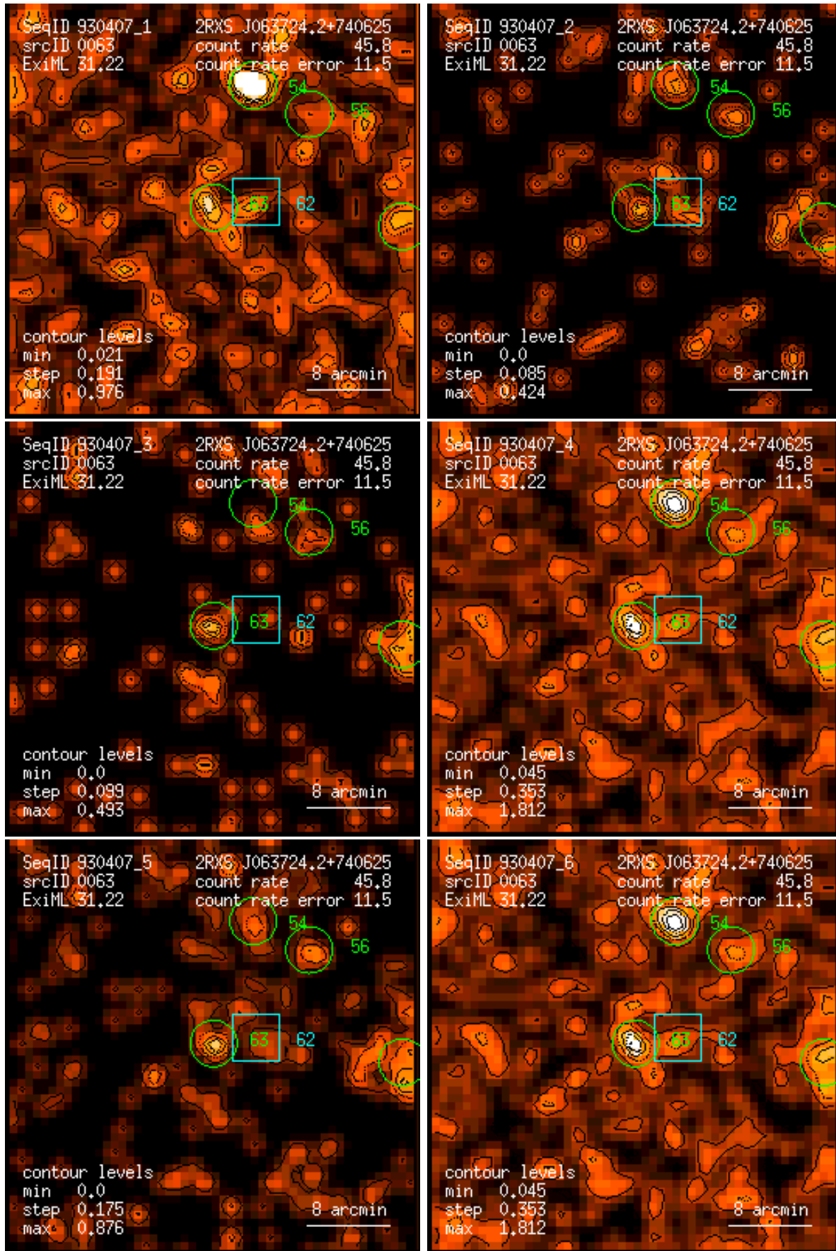
Figure 63: RASS 930407: detection 0063: band rate images, Gaussian filter: (1) PSPC channels 11 – 41, (2) 52 – 90, (3) 91 – 201, (4) 11 – 235, (5) 52 – 201, (6) 11 – 201. Broad band rates in counts/ks. Band rate contour levels in counts/ks/arcmin 2 .
