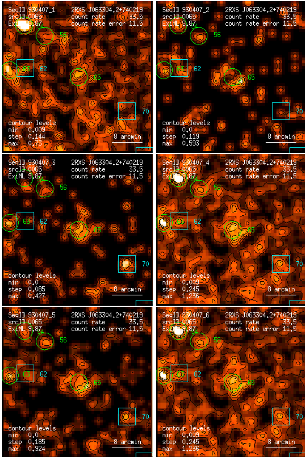
Figure 65: RASS 930407: detection 0065: band rate images, Gaussian filter: (1) PSPC channels 11 – 41, (2) 52 – 90, (3) 91 – 201, (4) 11 – 235, (5) 52 – 201, (6) 11 – 201. Broad band rates in counts/ks. Band rate contour levels in counts/ks/arcmin 2 .
