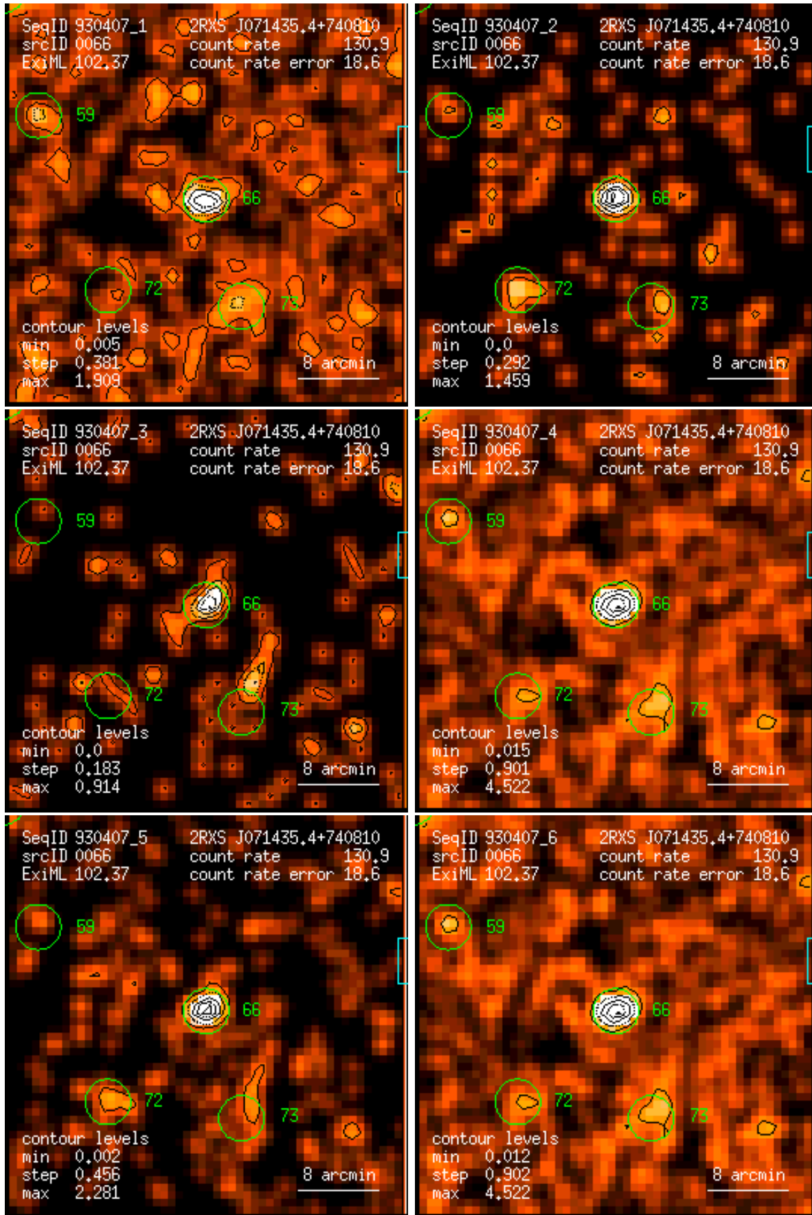
Figure 66: RASS 930407: detection 0066: band rate images, Gaussian filter: (1) PSPC channels 11 – 41, (2) 52 – 90, (3) 91 – 201, (4) 11 – 235, (5) 52 – 201, (6) 11 – 201. Broad band rates in counts/ks. Band rate contour levels in counts/ks/arcmin 2 .
