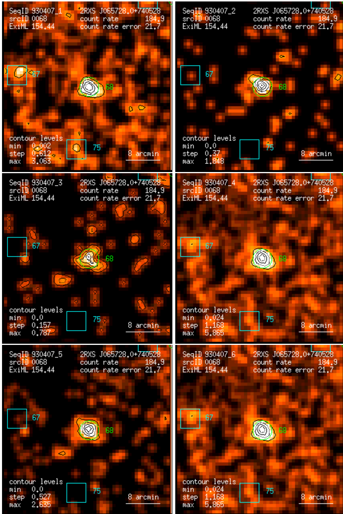
Figure 68: RASS 930407: detection 0068: band rate images, Gaussian filter: (1) PSPC channels 11 – 41, (2) 52 – 90, (3) 91 – 201, (4) 11 – 235, (5) 52 – 201, (6) 11 – 201. Broad band rates in counts/ks. Band rate contour levels in counts/ks/arcmin 2 .
