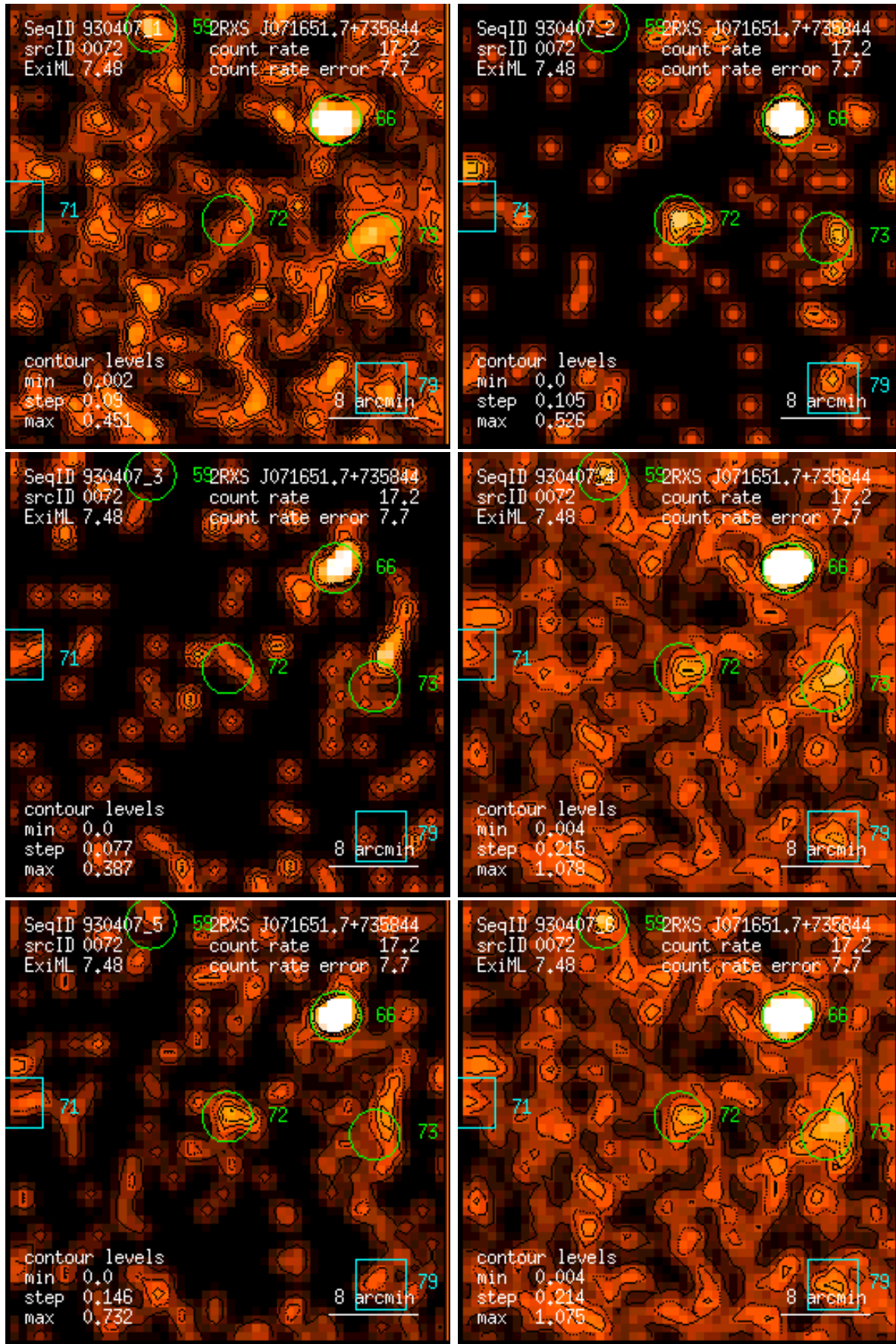
Figure 72: RASS 930407: detection 0072: band rate images, Gaussian filter: (1) PSPC channels 11 – 41, (2) 52 – 90, (3) 91 – 201, (4) 11 – 235, (5) 52 – 201, (6) 11 – 201. Broad band rates in counts/ks. Band rate contour levels in counts/ks/arcmin 2 .
