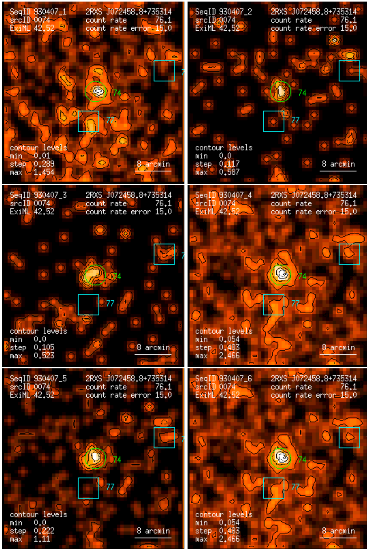
Figure 74: RASS 930407: detection 0074: band rate images, Gaussian filter: (1) PSPC channels 11 – 41, (2) 52 – 90, (3) 91 – 201, (4) 11 – 235, (5) 52 – 201, (6) 11 – 201. Broad band rates in counts/ks. Band rate contour levels in counts/ks/arcmin 2 .
