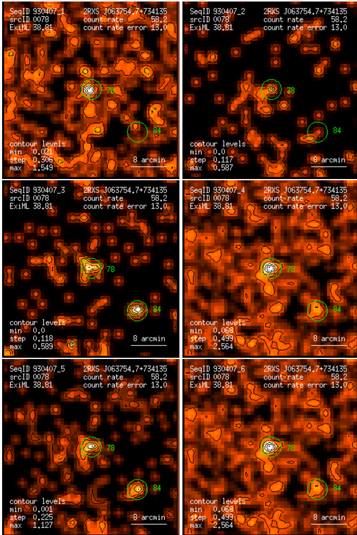
Figure 78: RASS 930407: detection 0078: band rate images, Gaussian filter: (1) PSPC channels 11 – 41, (2) 52 – 90, (3) 91 – 201, (4) 11 – 235, (5) 52 – 201, (6) 11 – 201. Broad band rates in counts/ks. Band rate contour levels in counts/ks/arcmin 2 .
