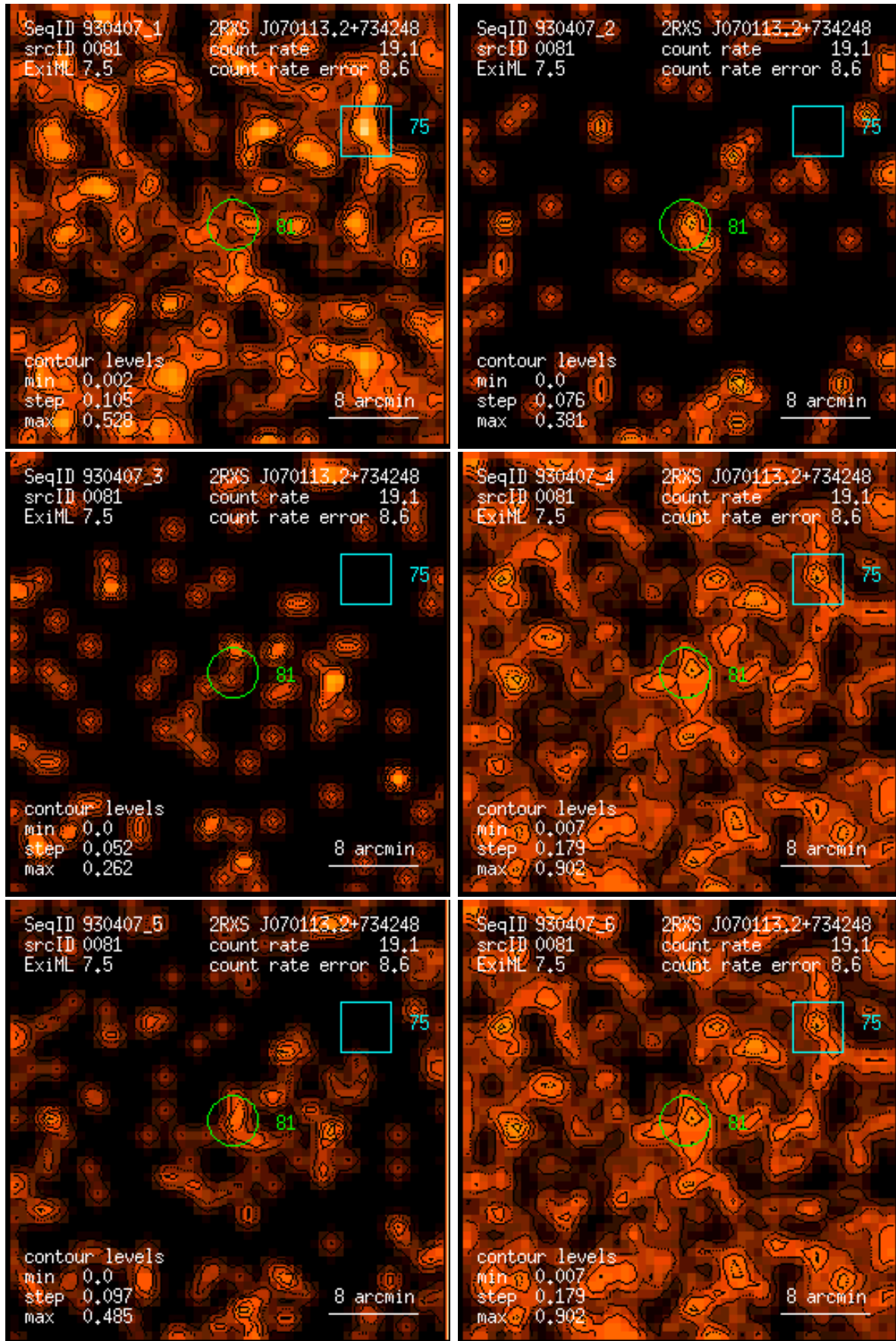
Figure 81: RASS 930407: detection 0081: band rate images, Gaussian filter: (1) PSPC channels 11 – 41, (2) 52 – 90, (3) 91 – 201, (4) 11 – 235, (5) 52 – 201, (6) 11 – 201. Broad band rates in counts/ks. Band rate contour levels in counts/ks/arcmin 2 .
