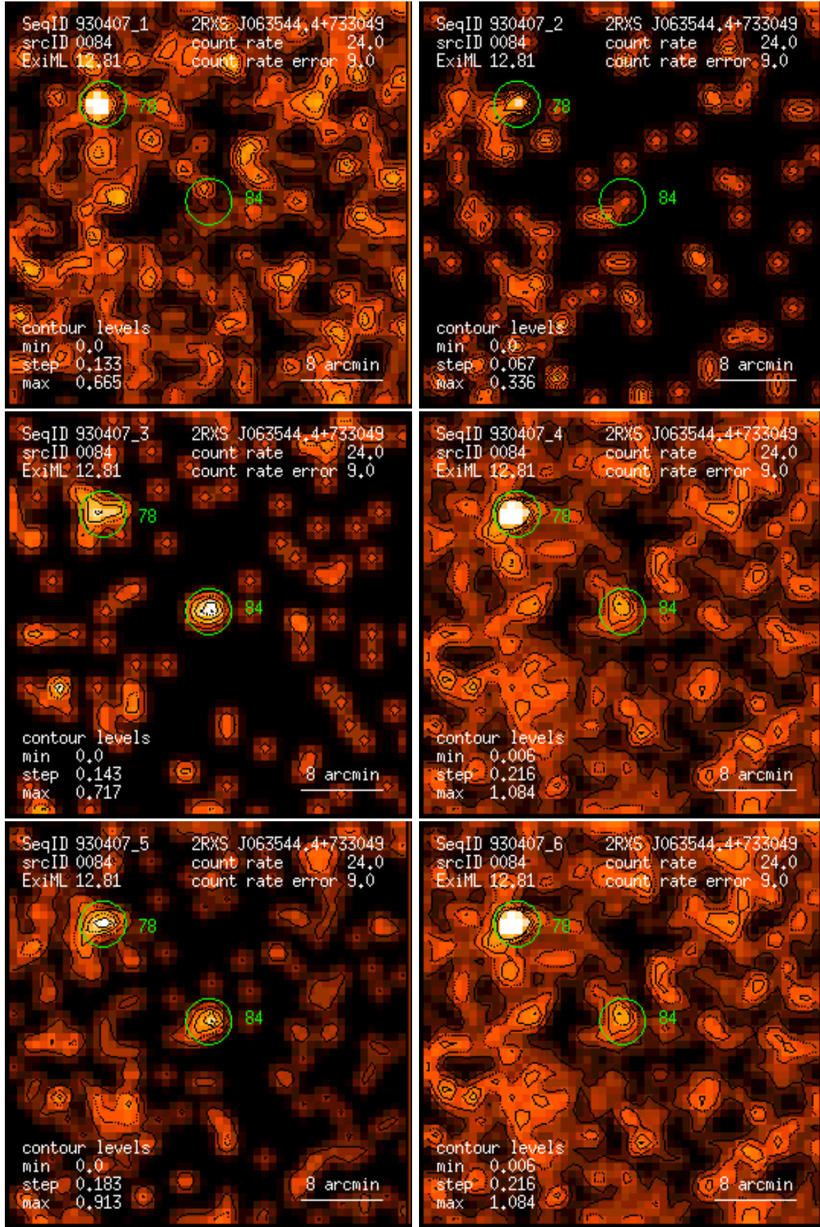
Figure 84: RASS 930407: detection 0084: band rate images, Gaussian filter: (1) PSPC channels 11 – 41, (2) 52 – 90, (3) 91 – 201, (4) 11 – 235, (5) 52 – 201, (6) 11 – 201. Broad band rates in counts/ks. Band rate contour levels in counts/ks/arcmin 2 .
