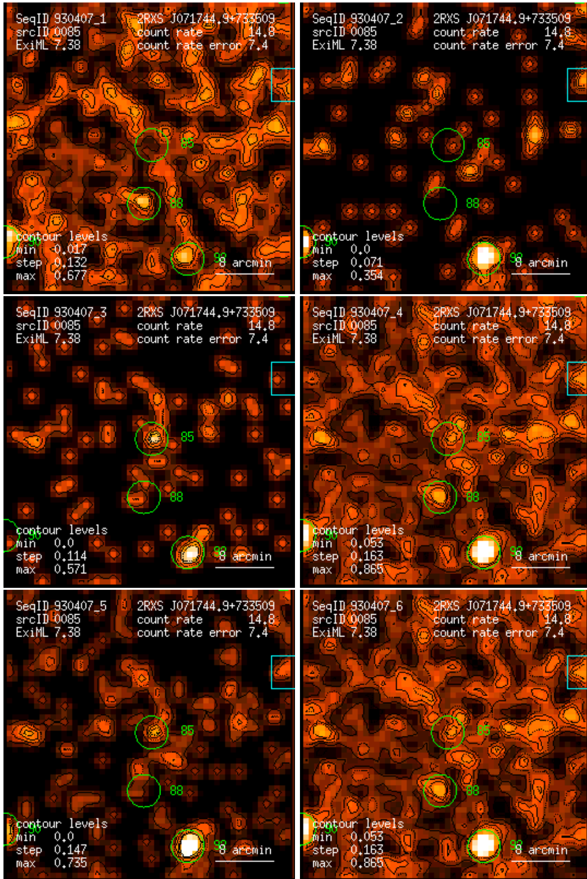
Figure 85: RASS 930407: detection 0085: band rate images, Gaussian filter: (1) PSPC channels 11 – 41, (2) 52 – 90, (3) 91 – 201, (4) 11 – 235, (5) 52 – 201, (6) 11 – 201. Broad band rates in counts/ks. Band rate contour levels in counts/ks/arcmin 2 .
