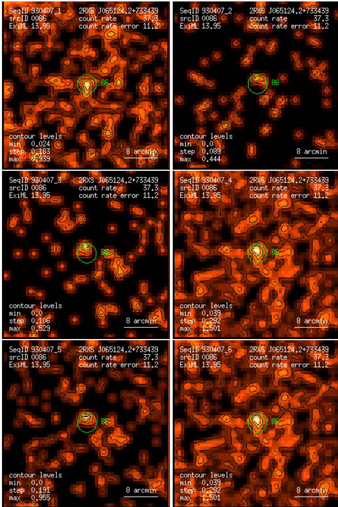
Figure 86: RASS 930407: detection 0086: band rate images, Gaussian filter: (1) PSPC channels 11 – 41, (2) 52 – 90, (3) 91 – 201, (4) 11 – 235, (5) 52 – 201, (6) 11 – 201. Broad band rates in counts/ks. Band rate contour levels in counts/ks/arcmin 2 .
