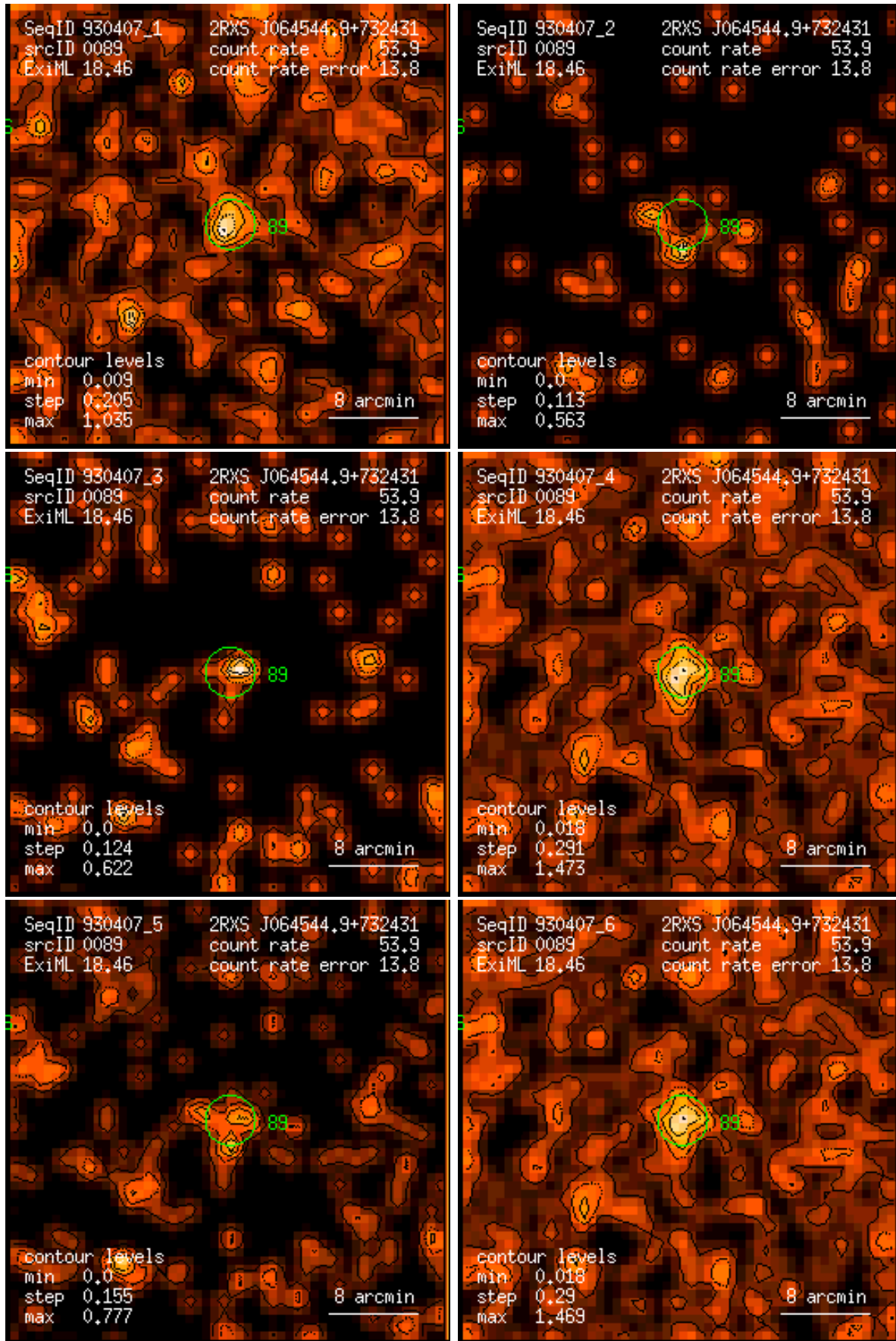
Figure 89: RASS 930407: detection 0089: band rate images, Gaussian filter: (1) PSPC channels 11 – 41, (2) 52 – 90, (3) 91 – 201, (4) 11 – 235, (5) 52 – 201, (6) 11 – 201. Broad band rates in counts/ks. Band rate contour levels in counts/ks/arcmin 2 .
