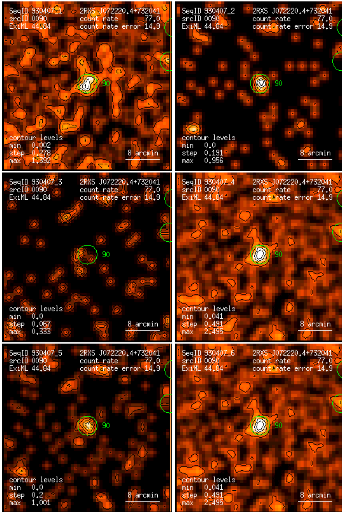
Figure 90: RASS 930407: detection 0090: band rate images, Gaussian filter: (1) PSPC channels 11 – 41, (2) 52 – 90, (3) 91 – 201, (4) 11 – 235, (5) 52 – 201, (6) 11 – 201. Broad band rates in counts/ks. Band rate contour levels in counts/ks/arcmin 2 .
