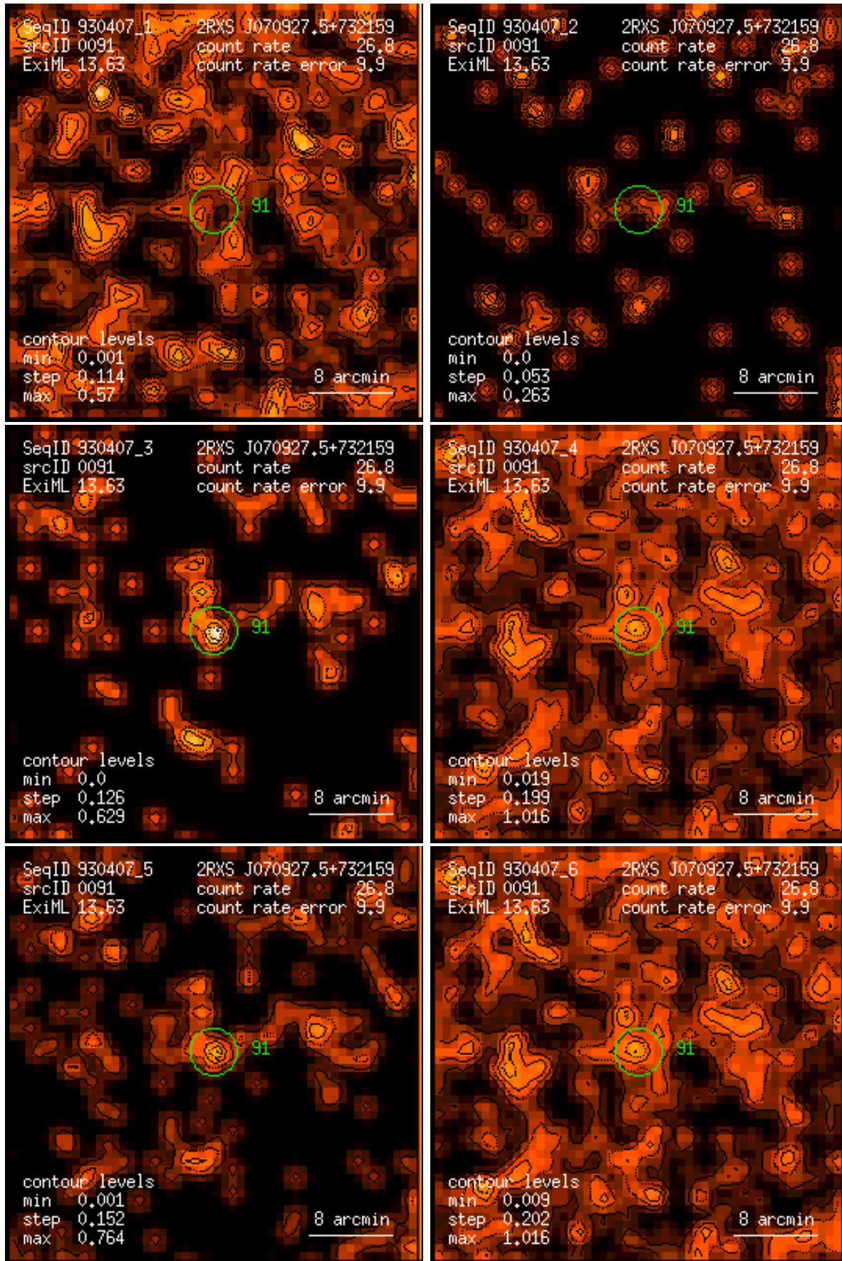
Figure 91: RASS 930407: detection 0091: band rate images, Gaussian filter: (1) PSPC channels 11 – 41, (2) 52 – 90, (3) 91 – 201, (4) 11 – 235, (5) 52 – 201, (6) 11 – 201. Broad band rates in counts/ks. Band rate contour levels in counts/ks/arcmin 2 .
