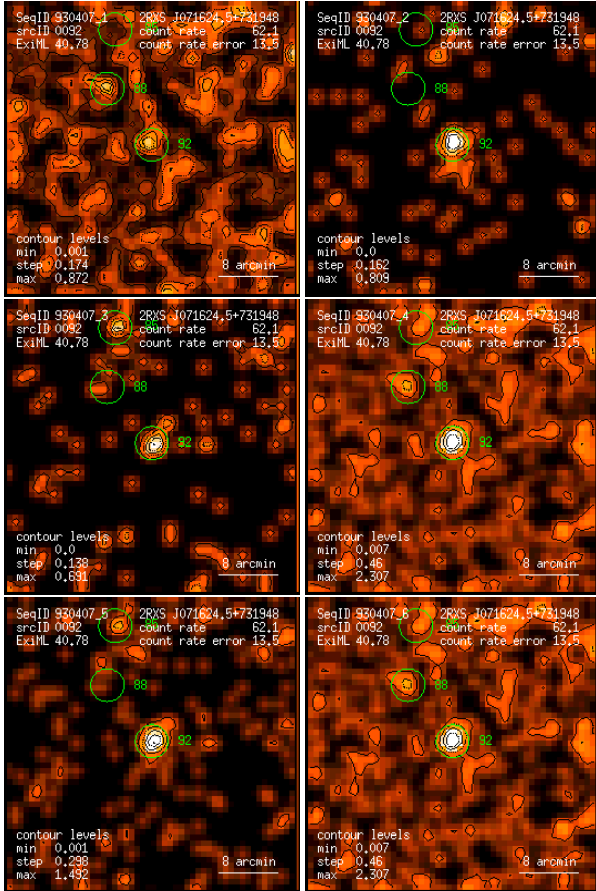
Figure 92: RASS 930407: detection 0092: band rate images, Gaussian filter: (1) PSPC channels 11 – 41, (2) 52 – 90, (3) 91 – 201, (4) 11 – 235, (5) 52 – 201, (6) 11 – 201. Broad band rates in counts/ks. Band rate contour levels in counts/ks/arcmin 2 .
