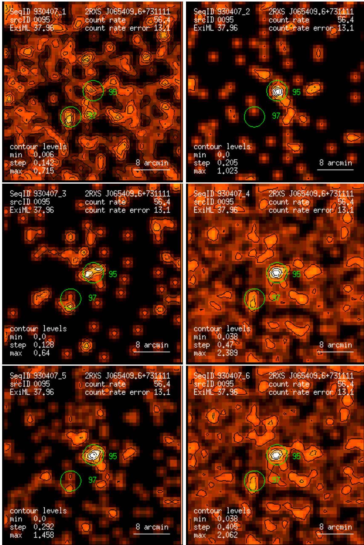
Figure 95: RASS 930407: detection 0095: band rate images, Gaussian filter: (1) PSPC channels 11 – 41, (2) 52 – 90, (3) 91 – 201, (4) 11 – 235, (5) 52 – 201, (6) 11 – 201. Broad band rates in counts/ks. Band rate contour levels in counts/ks/arcmin 2 .
