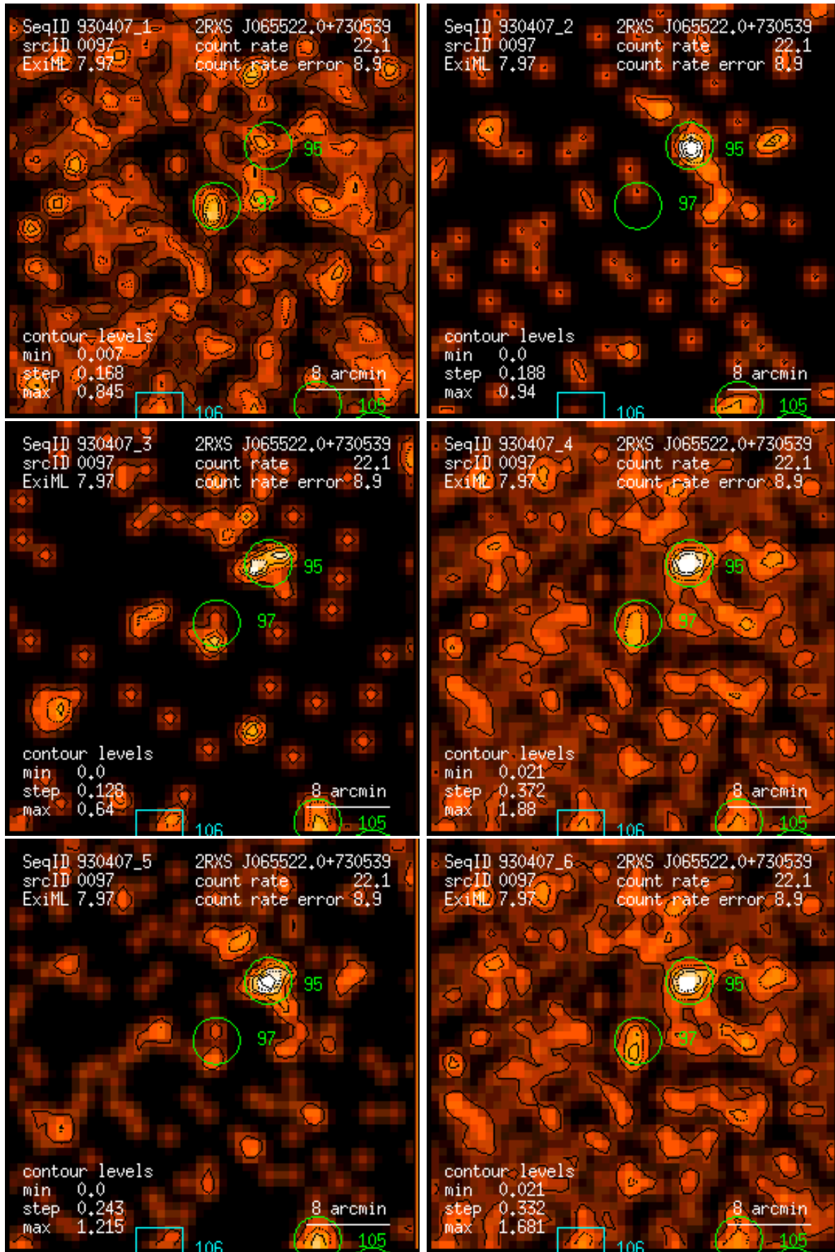
Figure 97: RASS 930407: detection 0097: band rate images, Gaussian filter: (1) PSPC channels 11 – 41, (2) 52 – 90, (3) 91 – 201, (4) 11 – 235, (5) 52 – 201, (6) 11 – 201. Broad band rates in counts/ks. Band rate contour levels in counts/ks/arcmin 2 .
