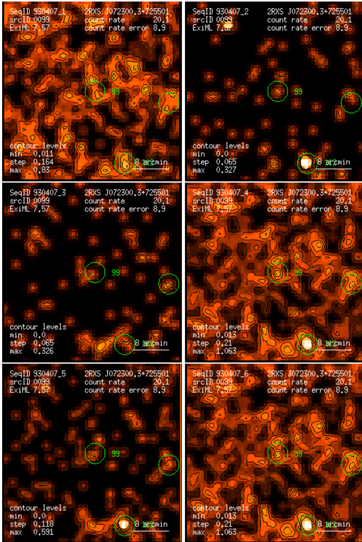
Figure 99: RASS 930407: detection 0099: band rate images, Gaussian filter: (1) PSPC channels 11 – 41, (2) 52 – 90, (3) 91 – 201, (4) 11 – 235, (5) 52 – 201, (6) 11 – 201. Broad band rates in counts/ks. Band rate contour levels in counts/ks/arcmin 2 .
