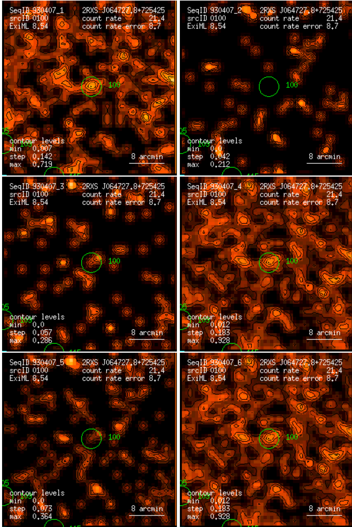
Figure 100: RASS 930407: detection 0100: band rate images, Gaussian filter: (1) PSPC channels 11 – 41, (2) 52 – 90, (3) 91 – 201, (4) 11 – 235, (5) 52 – 201, (6) 11 – 201. Broad band rates in counts/ks. Band rate contour levels in counts/ks/arcmin 2 .
