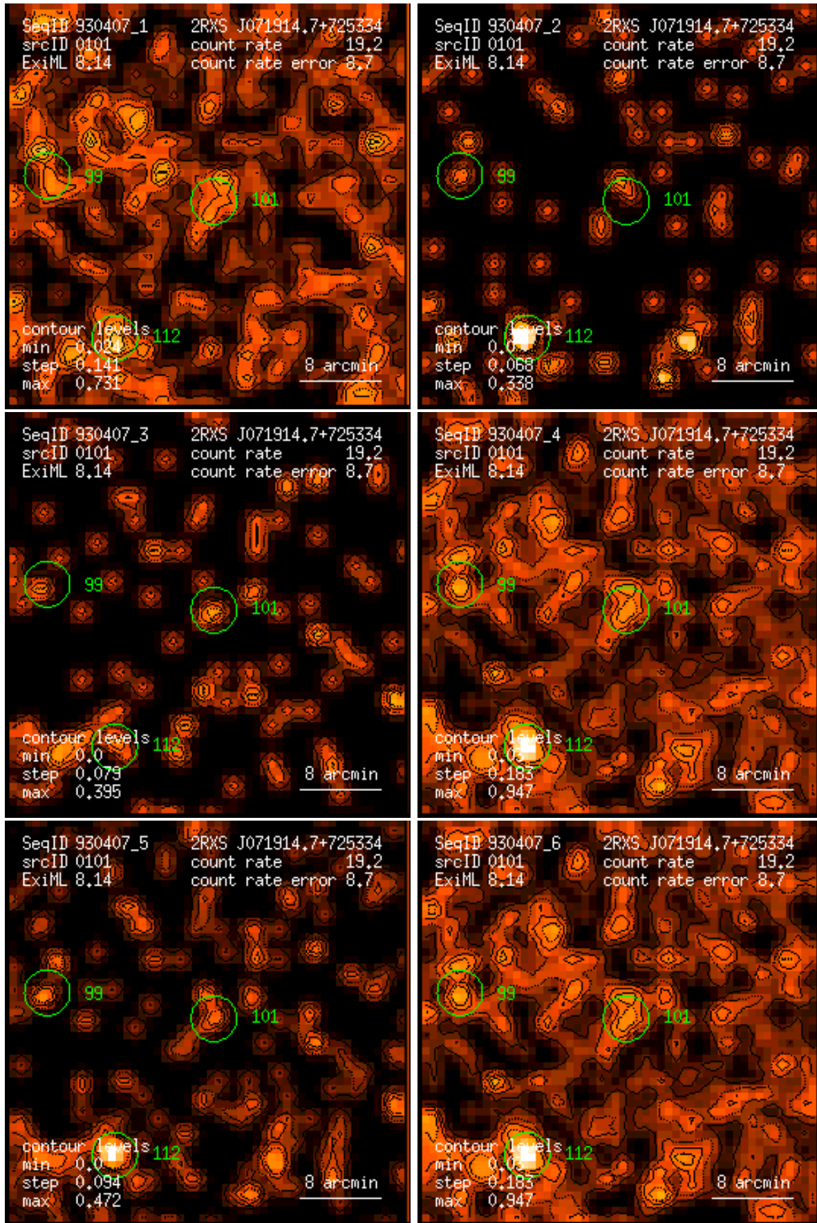
Figure 101: RASS 930407: detection 0101: band rate images, Gaussian filter: (1) PSPC channels 11 – 41, (2) 52 – 90, (3) 91 – 201, (4) 11 – 235, (5) 52 – 201, (6) 11 – 201. Broad band rates in counts/ks. Band rate contour levels in counts/ks/arcmin 2 .
