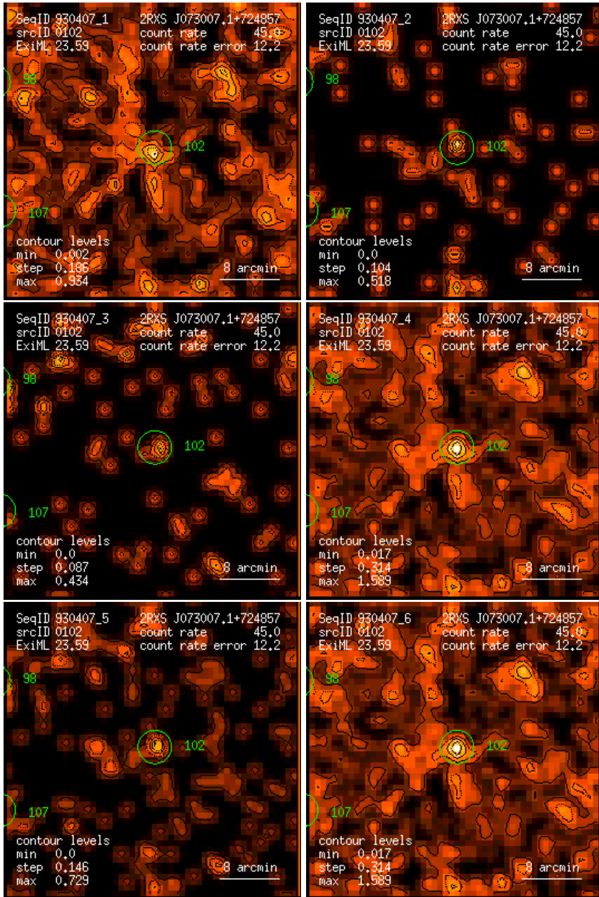
Figure 102: RASS 930407: detection 0102: band rate images, Gaussian filter: (1) PSPC channels 11 – 41, (2) 52 – 90, (3) 91 – 201, (4) 11 – 235, (5) 52 – 201, (6) 11 – 201. Broad band rates in counts/ks. Band rate contour levels in counts/ks/arcmin 2 .
